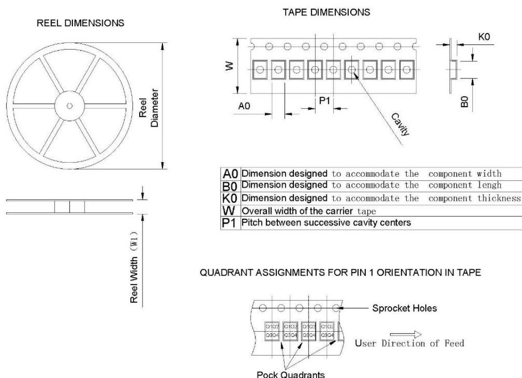
Figure 7. Package
