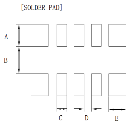
Figure 4. Recommended Solder Pad
