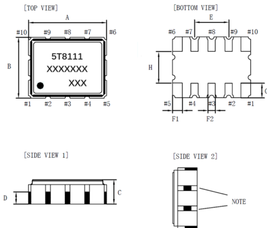
Figure 3. Dimensions
