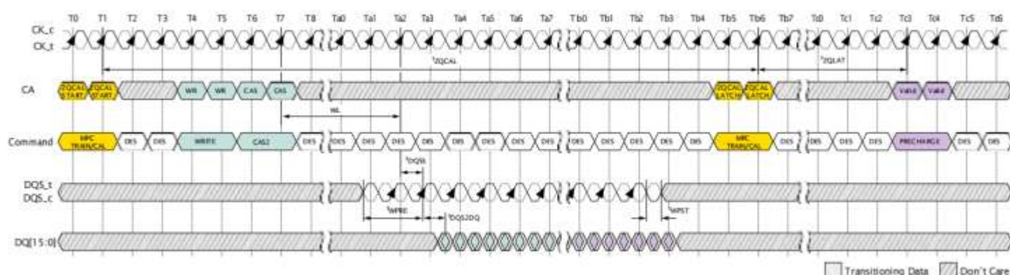
Figure I38: ZQCAL Timing
