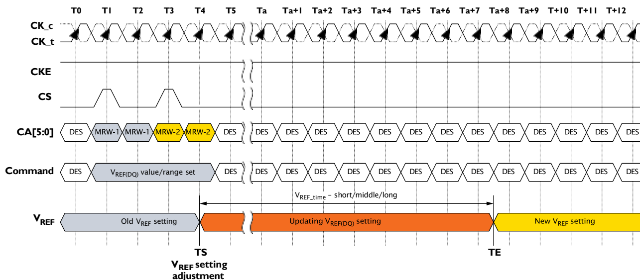
Figure 110: V_{REF(DQ)} Transition Time for Short, Middle, or Long Changes
