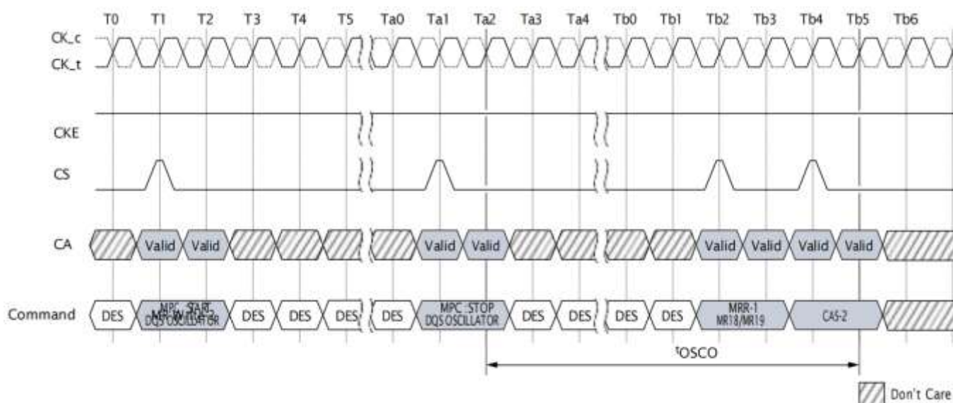
Figure I35: In Case of DQS Interval Oscillator is Stopped by MPC Command
