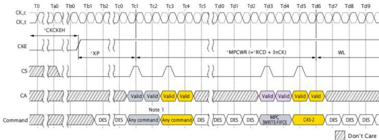
Figure 133: Power-Down Exit to MPC[WRITE-FIFO] Timing
