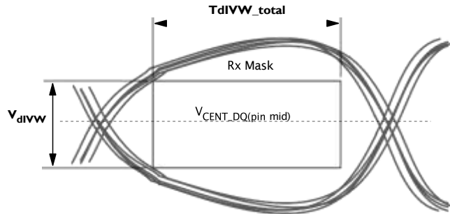
Figure 176: DQ Receiver (Rx) Mask
