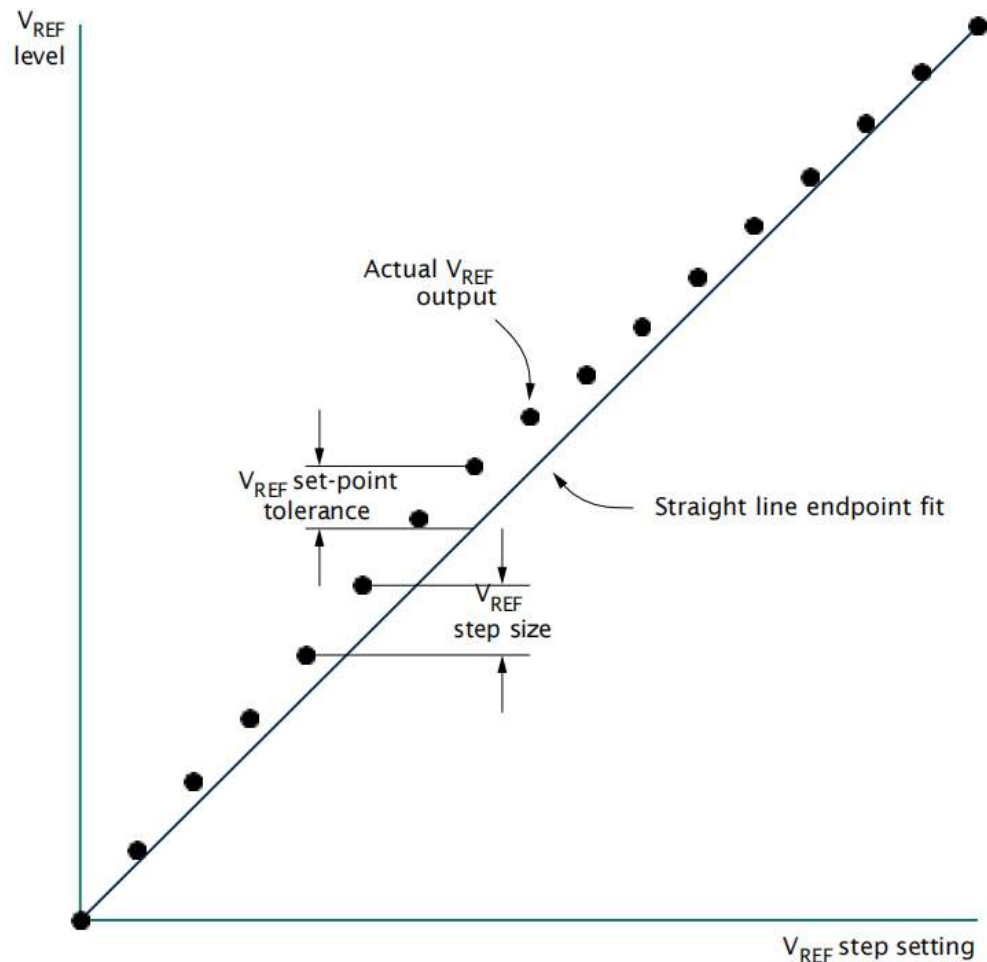
Figure 109: V_{REF} Set Tolerance and Step Size
