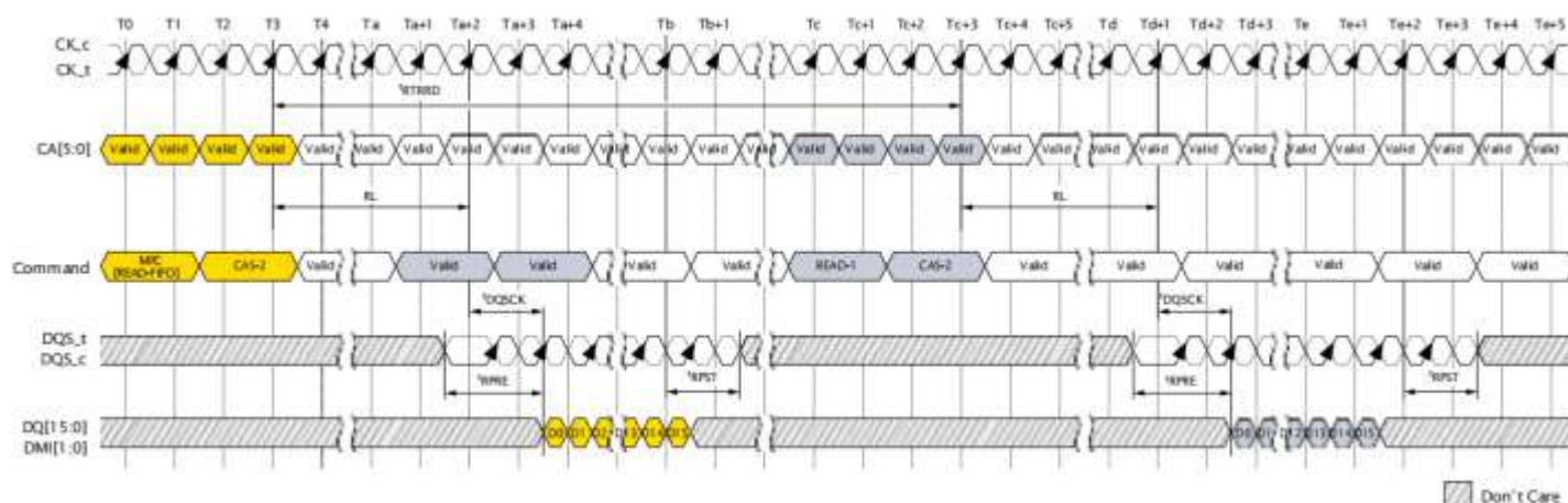
Figure 125: READ-FIFO – t_{RPRE} = \text{Toggle} , t_{RPST} = 1.5nCK
