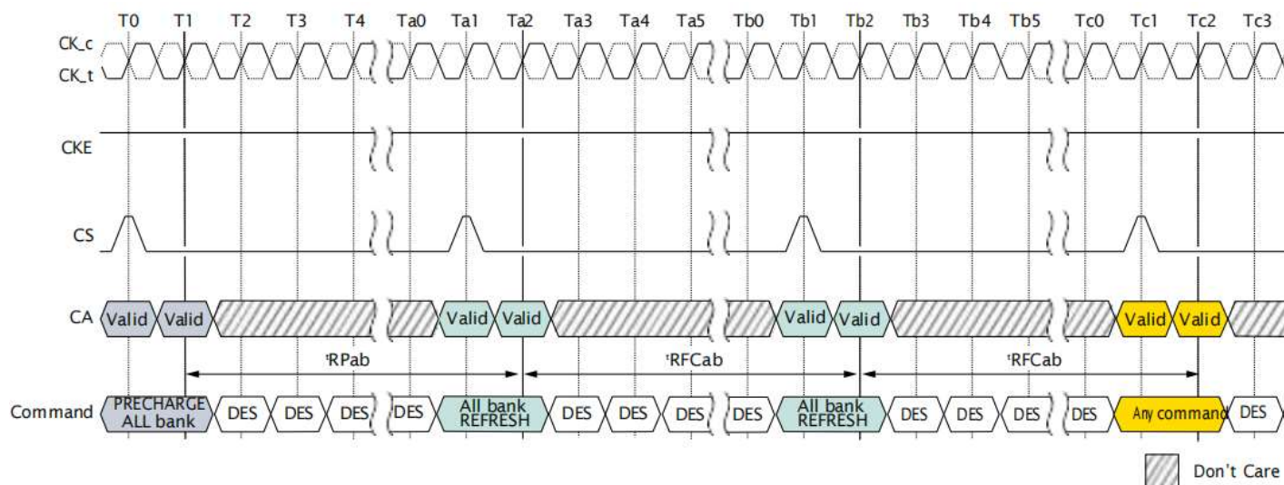
Figure 73: All-Bank REFRESH Operation
