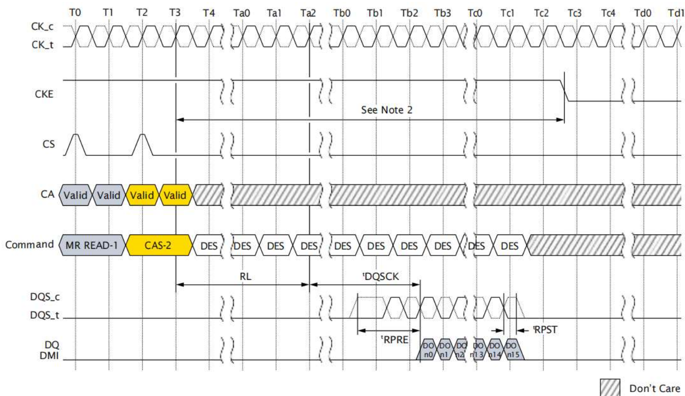
Figure 9I: Mode Register Read to Power-Down Entry
