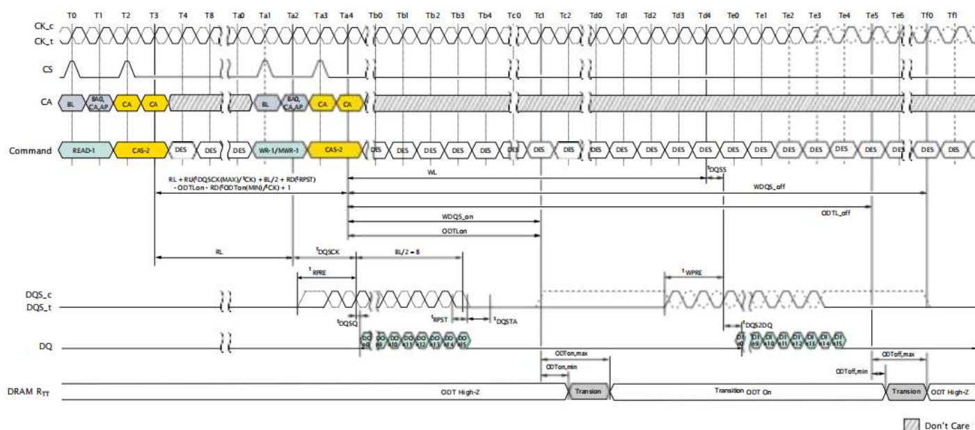
Figure 4I: Burst READ Followed by Burst WRITE or Burst MASKED WRITE (ODT Enable)
