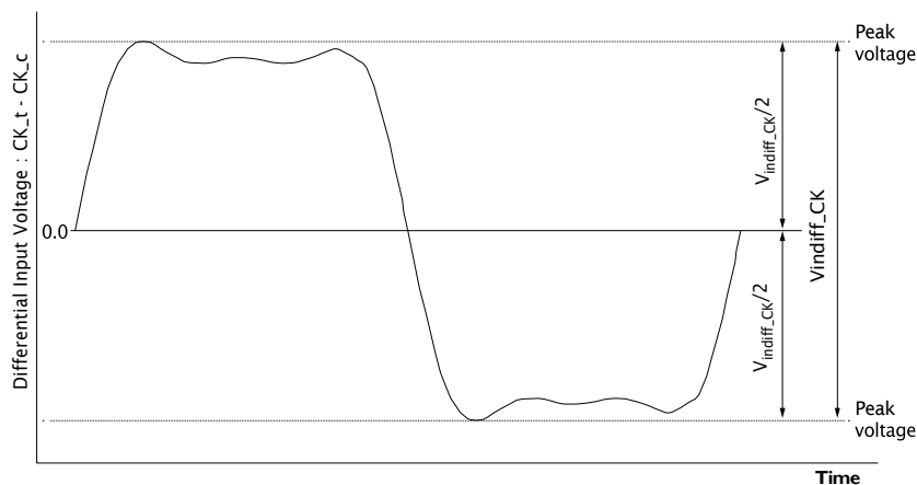
Figure I52: CK Differential Input Voltage
