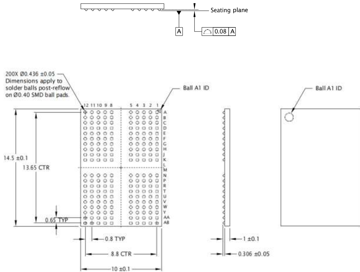
Figure 9: 200-Ball TFBGA – 10mm x 14.5mm x 1.1mm
