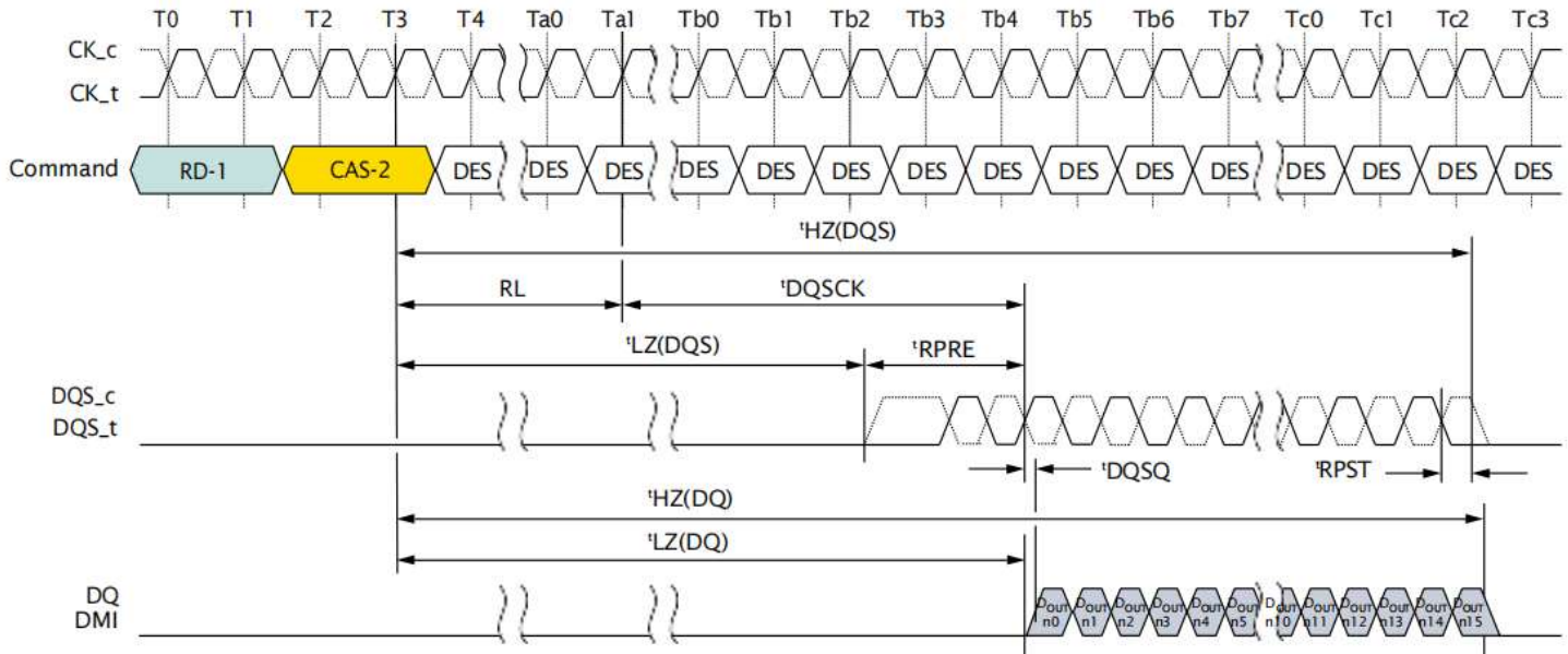
Figure 24: Read Timing
