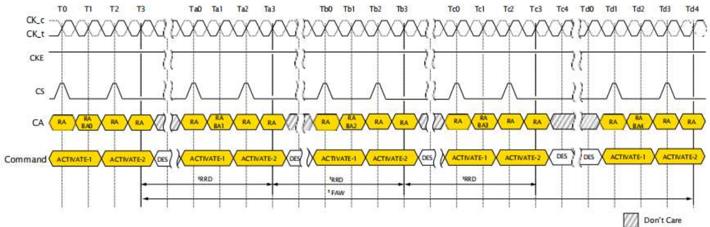
Figure 16: t_{FAW} Timing
