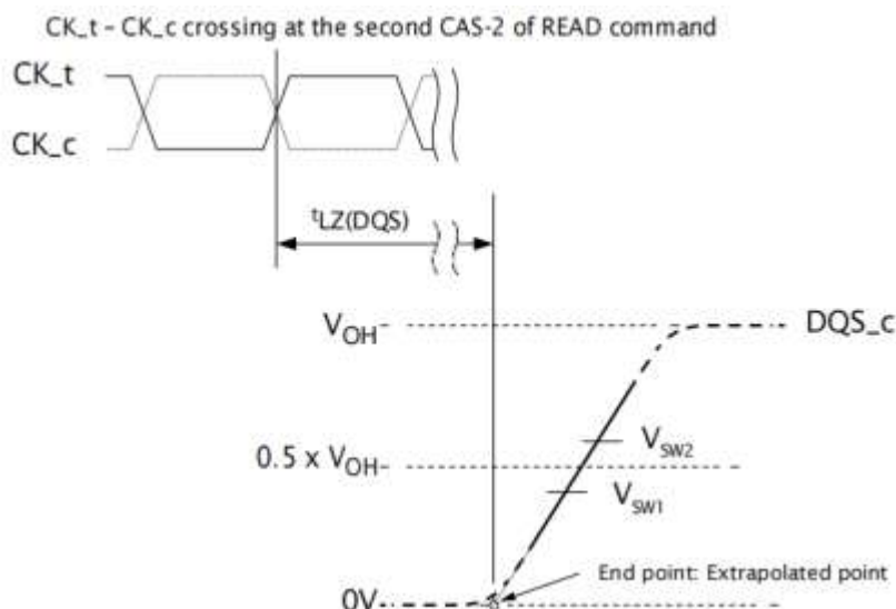
Figure 181: t_{LZ}(DQS) Method for Calculating Transitions and Endpoint
