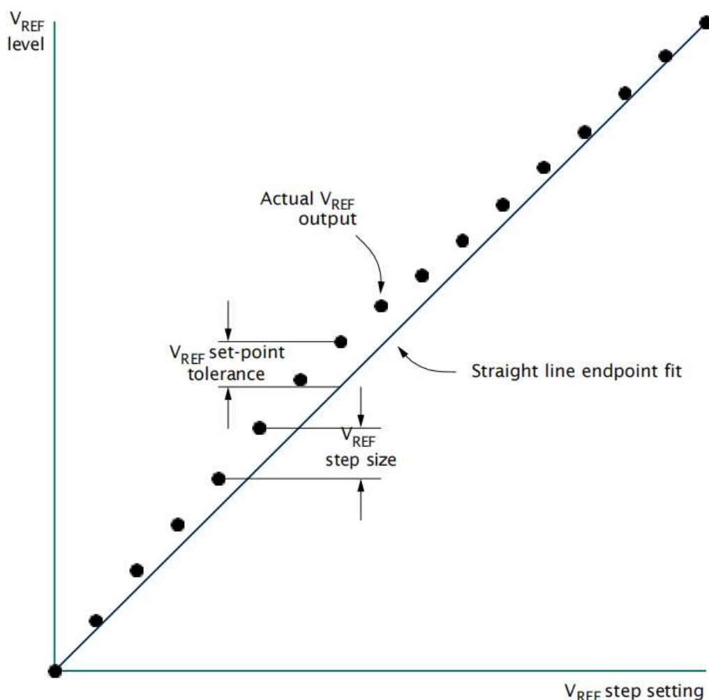
Figure I02: V_{REF} Set-Point Tolerance and Step Size
