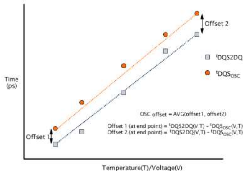
Figure I34: Interval Oscillator Offset – OSC_{offset}
