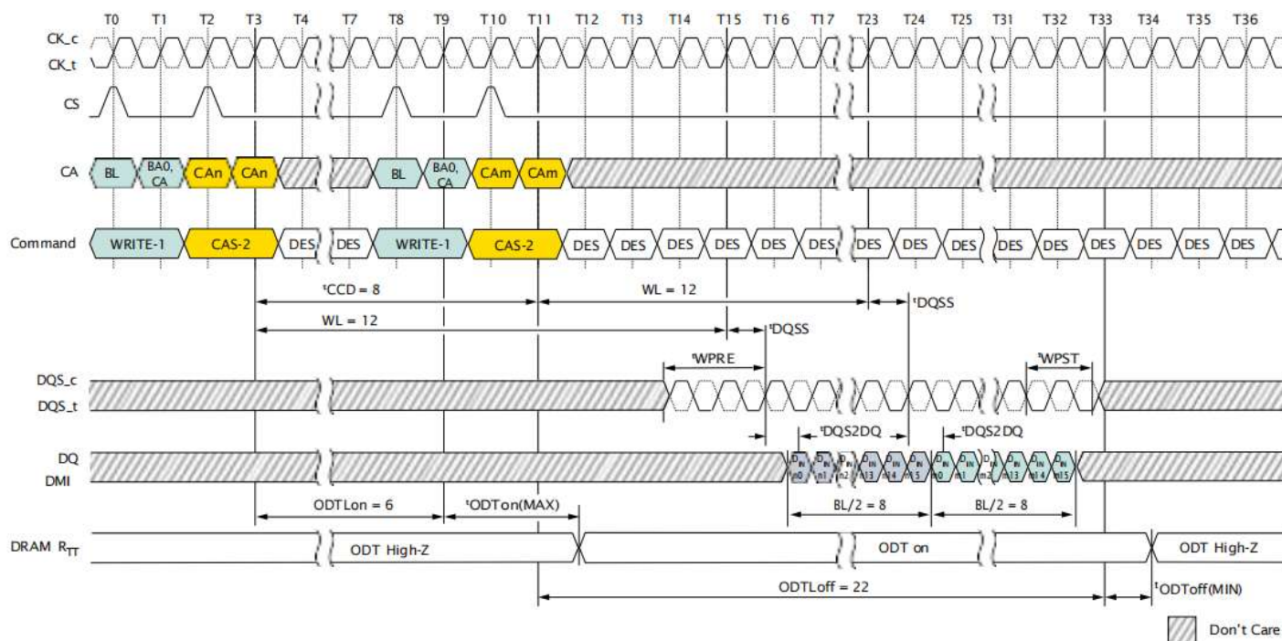
Figure 56: Seamless WRITE: t_{CCD} = \text{MIN} , 1.5nCK Postamble, 533 MHz < Clock Frequency \leq 800 MHz, ODT Worst Timing Case
