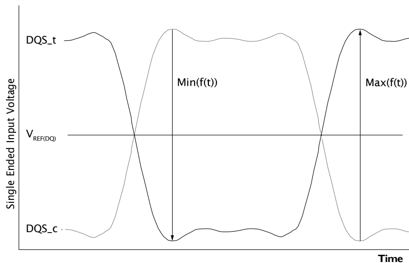
Figure I58: Definition of Differential DQS Peak Voltage
