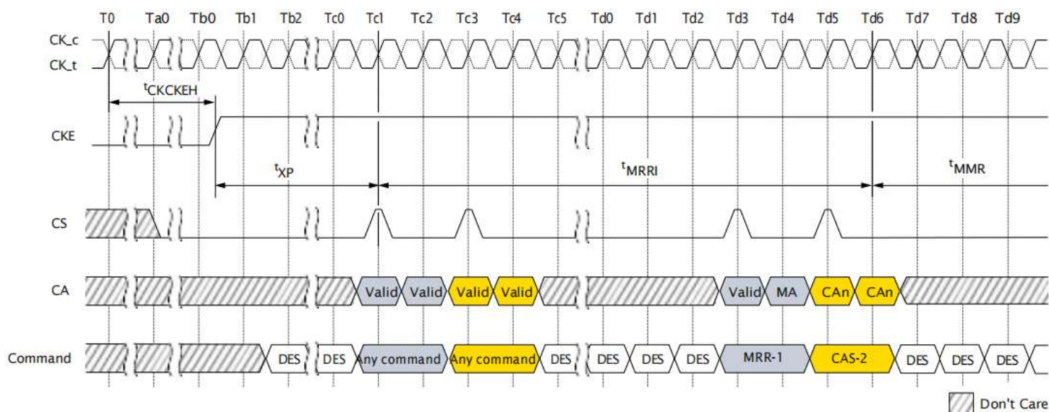
Figure 97: MRR Following Power-Down
