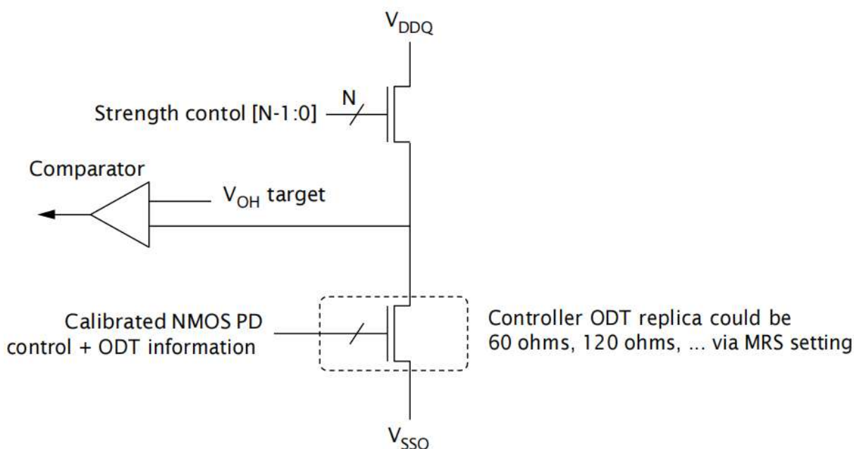
Figure 167: Pull-Up Calibration
