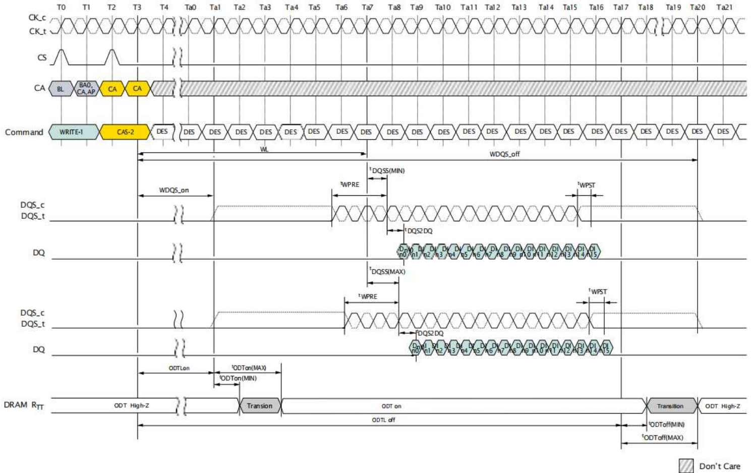
Figure 39: Burst WRITE Operation
