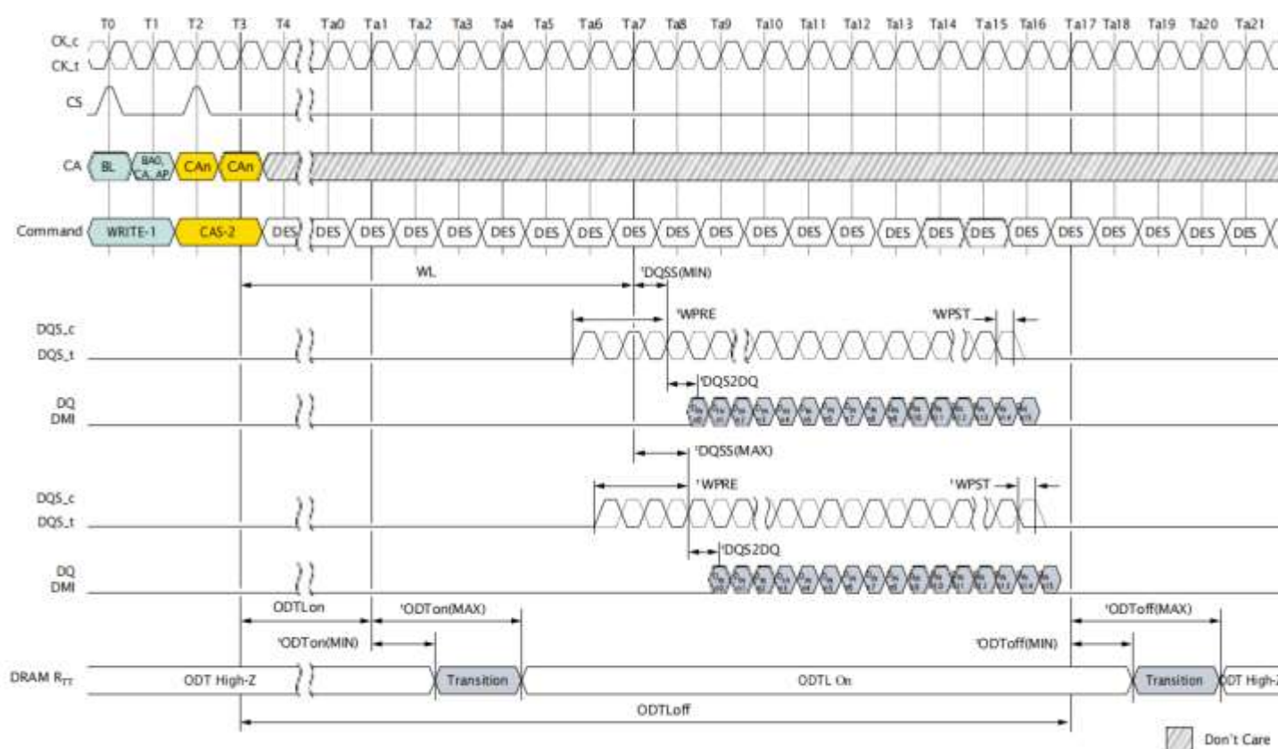
Figure 146: Asynchronous ODTon/ODT off Timing
