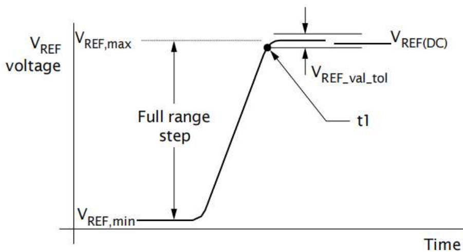
Figure 114: V_{REF(DQ)} Full Step from V_{REF,max} to V_{REF,min}
