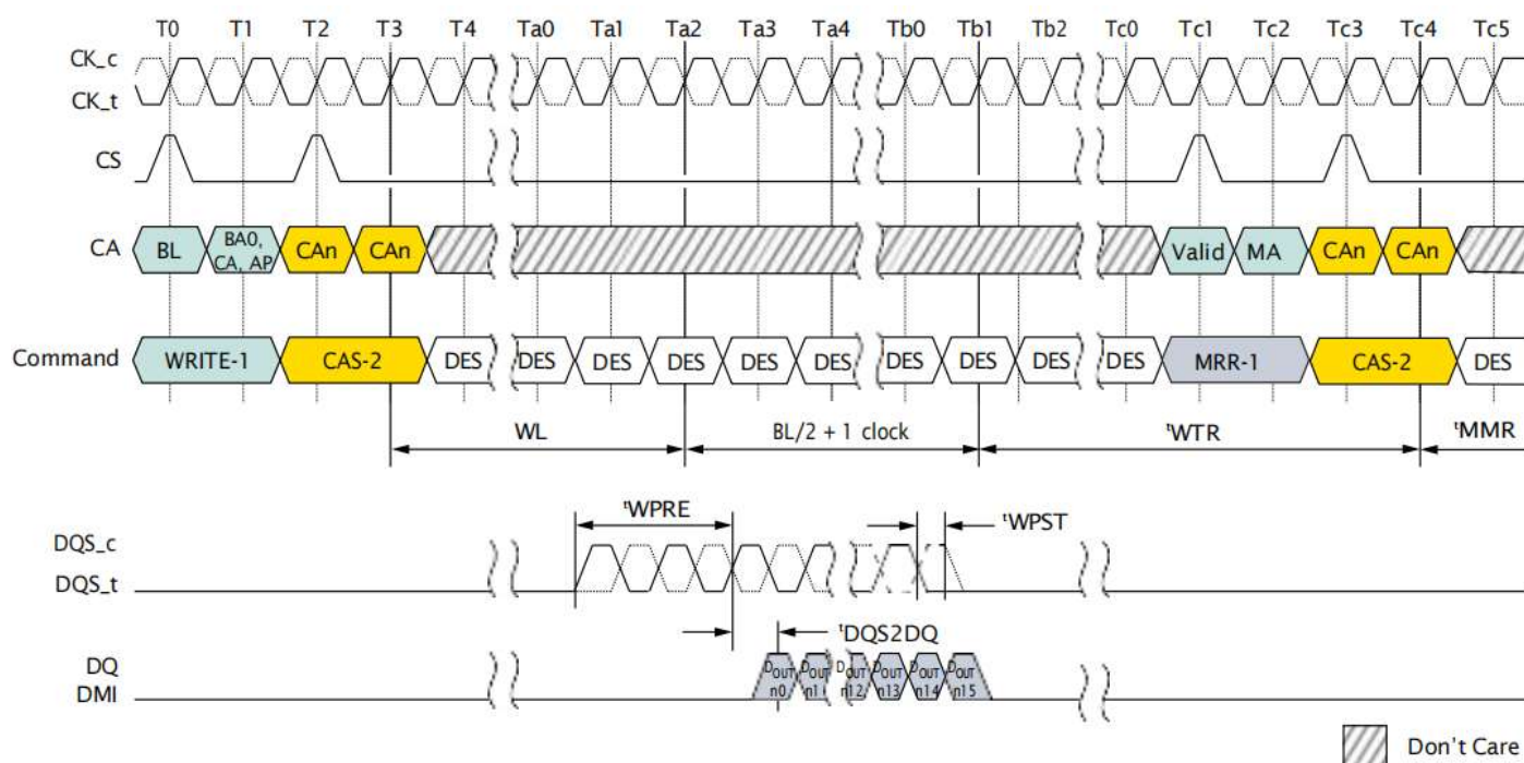
Figure 96: WRITE-to-MRR Timing
