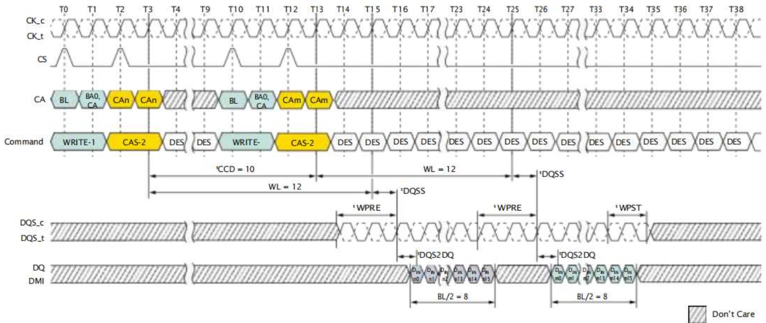
Figure 61: Consecutive WRITE: t_{CCD} = MIN + 2 , 1.5nCK Postamble
