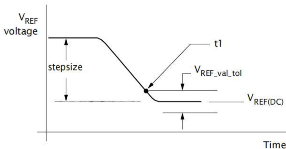
Figure I06: V_{REF(CA)} Full Step from V_{REF,min} to V_{REF,max}
