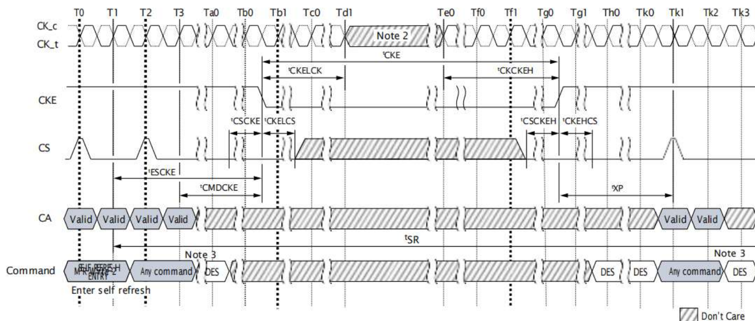
Figure 8I: Command Input Timings after Power-Down Exit During Self Refresh
