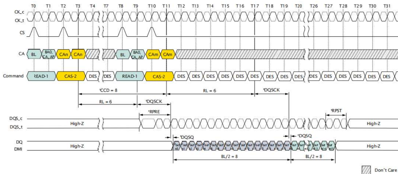
Figure 42: READ Operations: t_{CCD} = \text{MIN} , Preamble = Toggle, 1.5nCK Postamble
