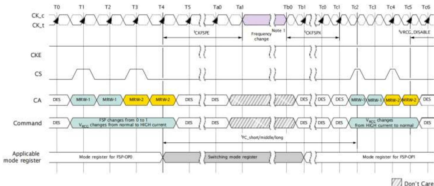
Figure I39: Frequency Set Point Switching Timing
