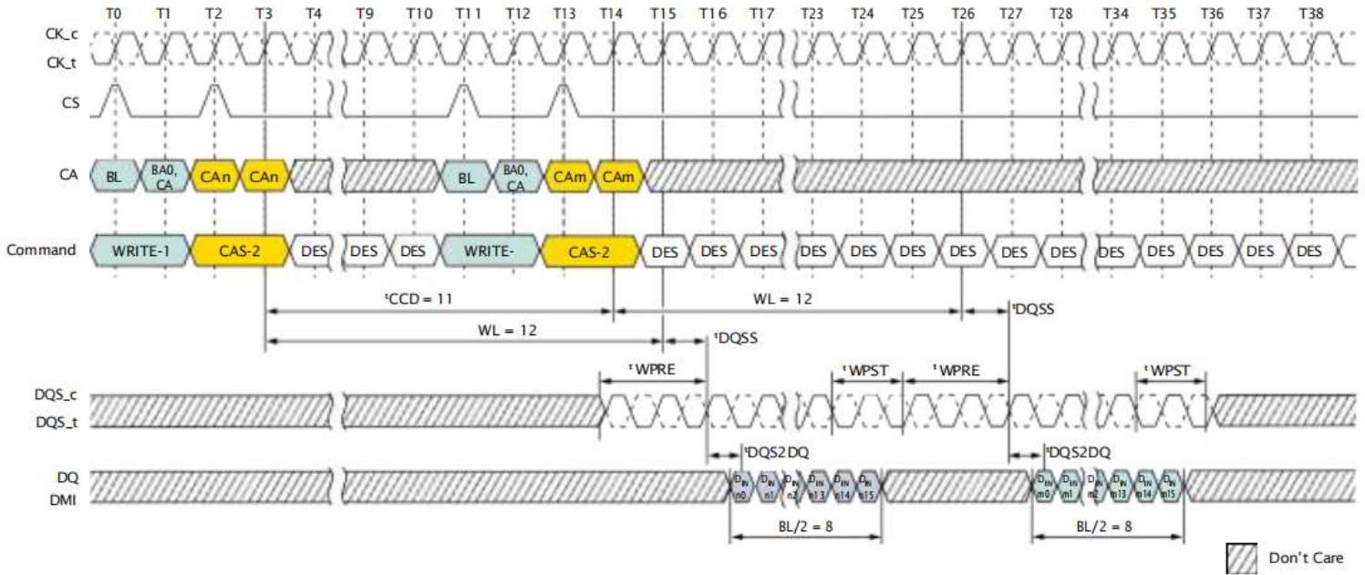
Figure 63: Consecutive WRITE: t_{CCD} = \text{MIN} + 3, 1.5n\text{CK} Postamble
