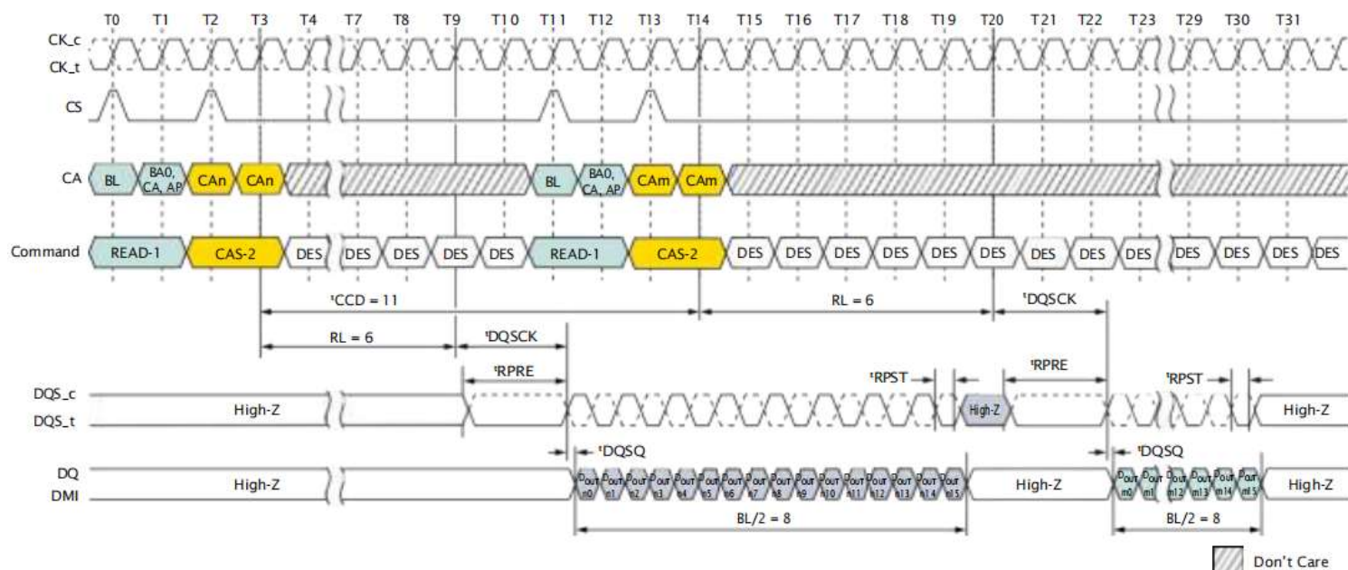
Figure 54: Consecutive READ: t_{CCD} = MIN + 3 , Preamble = Static, 0.5nCK Postamble
