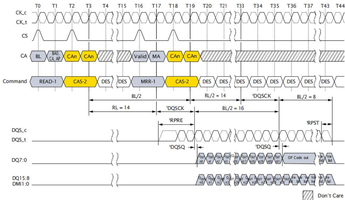
Figure 95: READ-to-MRR Timing
