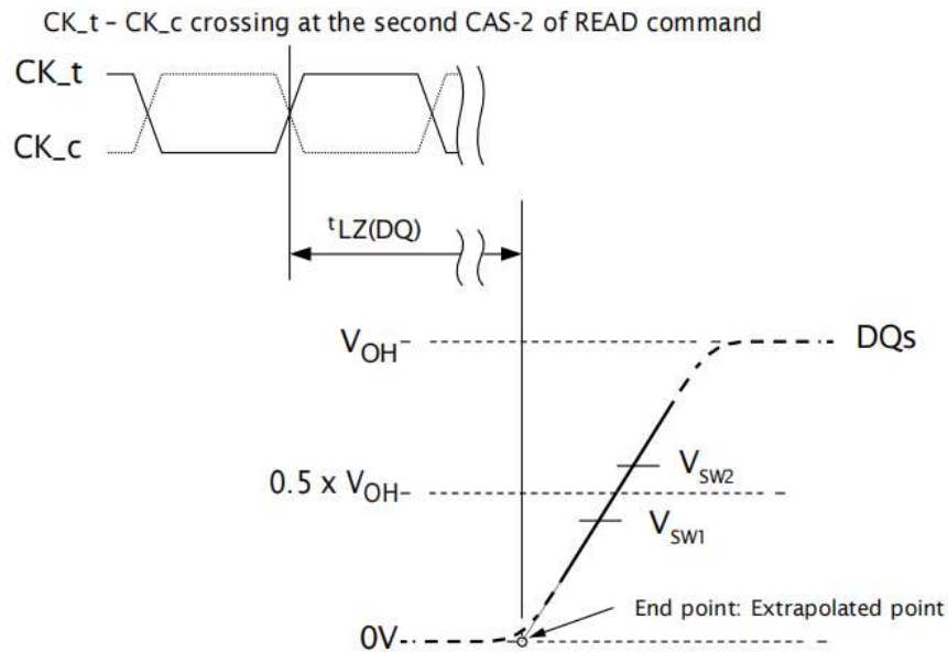
Figure 183: t_{LZ}(DQ) Method for Calculating Transitions and Endpoint
