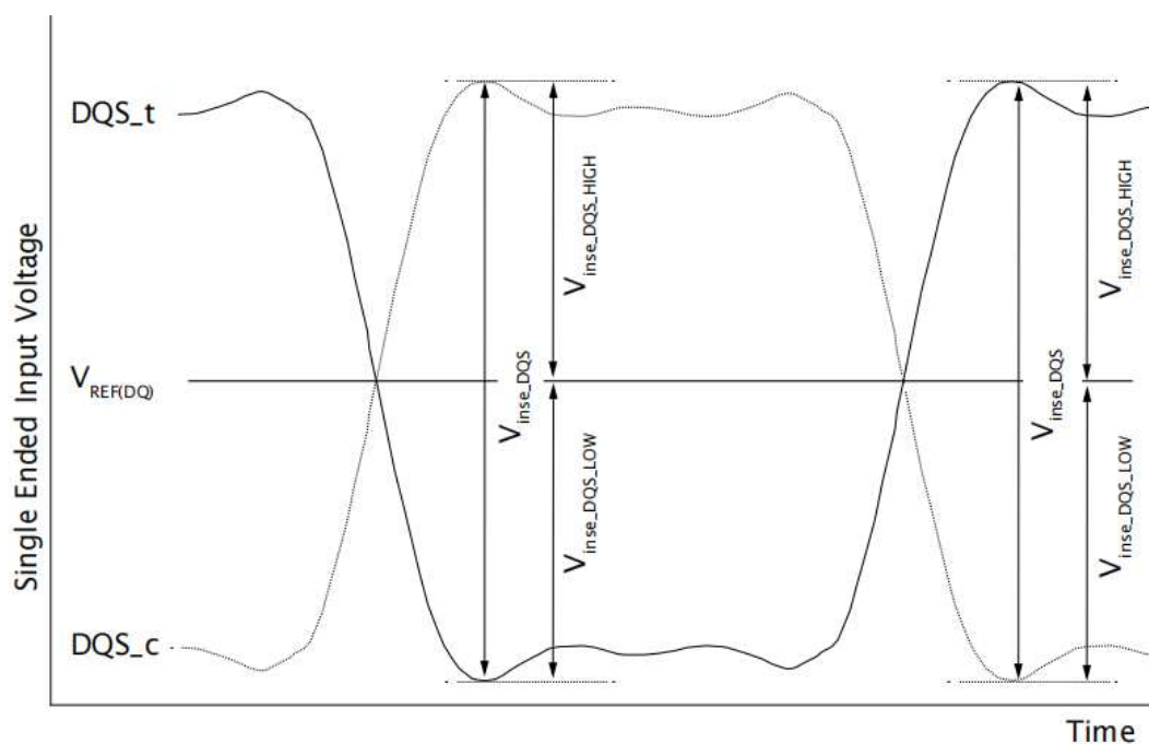
Figure I59: DQS Single-Ended Input Voltage
