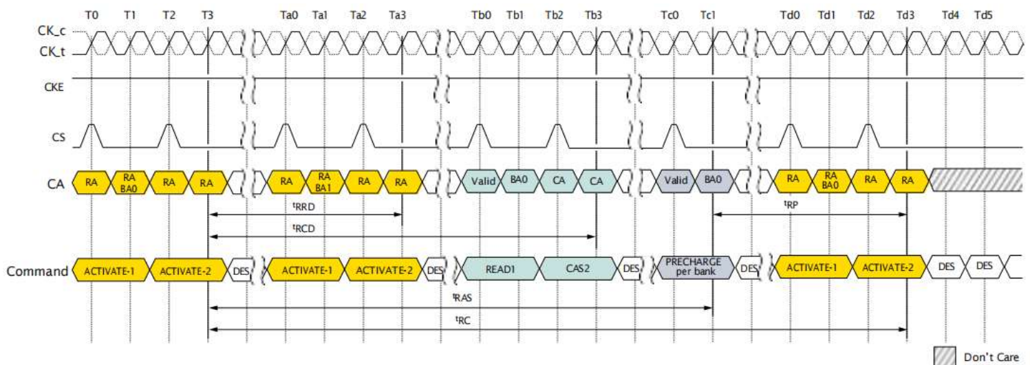
Figure 15: ACTIVATE Command
