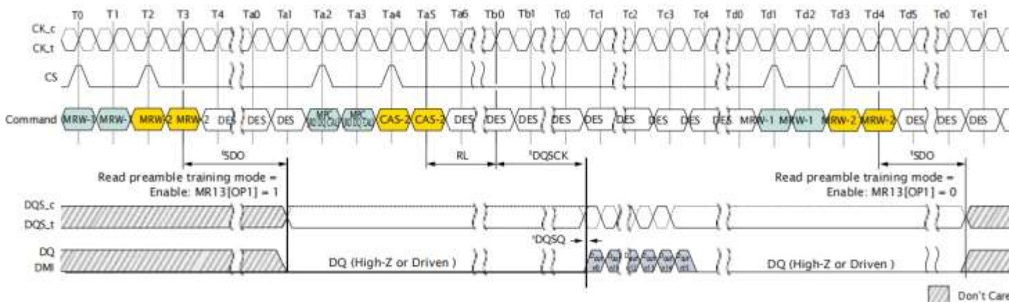
Figure 149: Read Preamble Training
