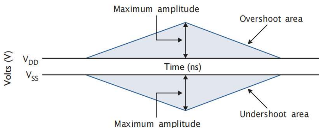
Figure 164: Overshoot and Undershoot Definition
