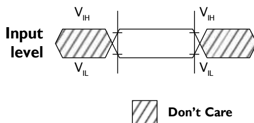
Figure I 51: Input Timing Definition for RESET_n
