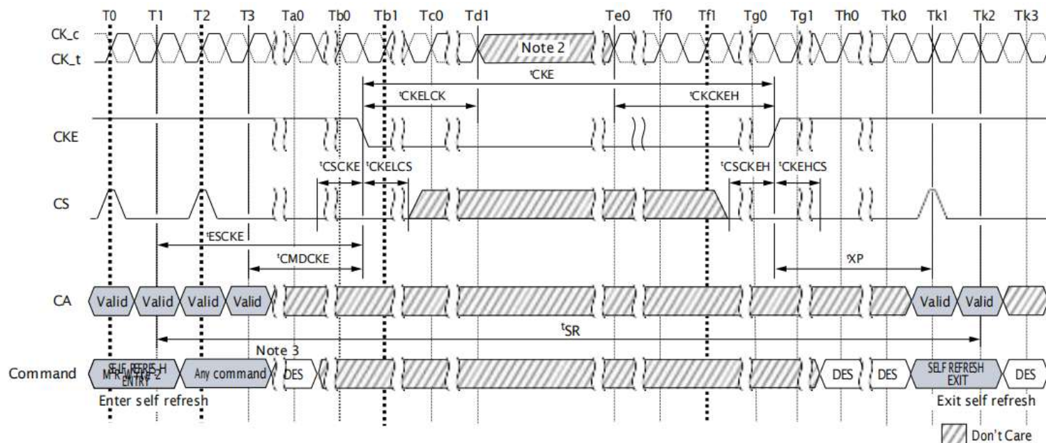
Figure 80: Self Refresh Entry/Exit Timing with Power-Down Entry/Exit
