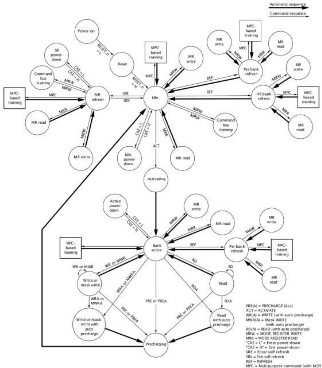
Figure 12: Simplified State Diagram
