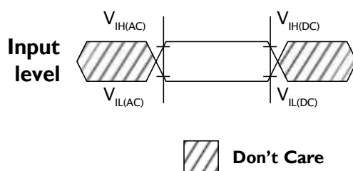
Figure I 50: Input Timing Definition for CKE
