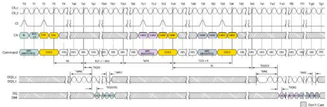
Figure 130: MPC[WRITE-FIFO]-to-MPC[READ-FIFO] Timing
