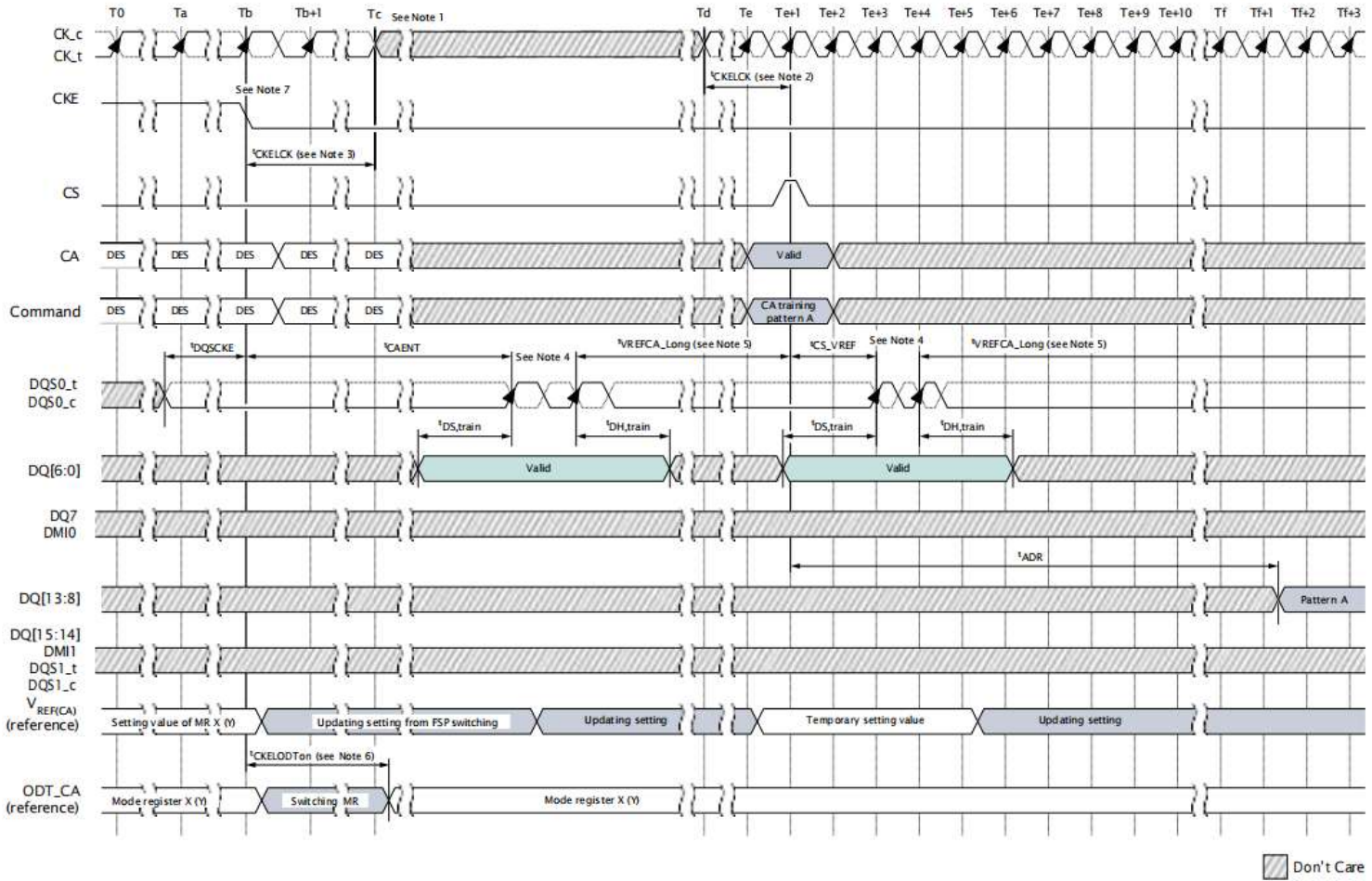
Figure I I6: Consecutive V_{REF(CA)} Value Update
