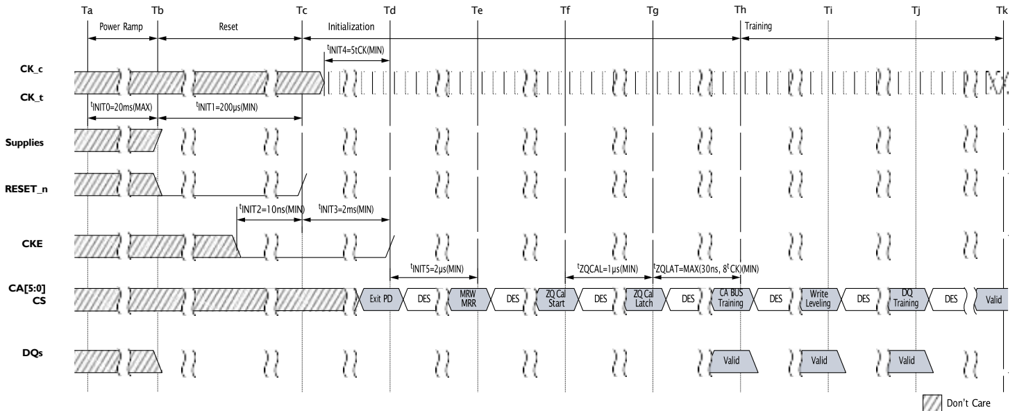
Figure 14: Voltage Ramp and Initialization Sequence
