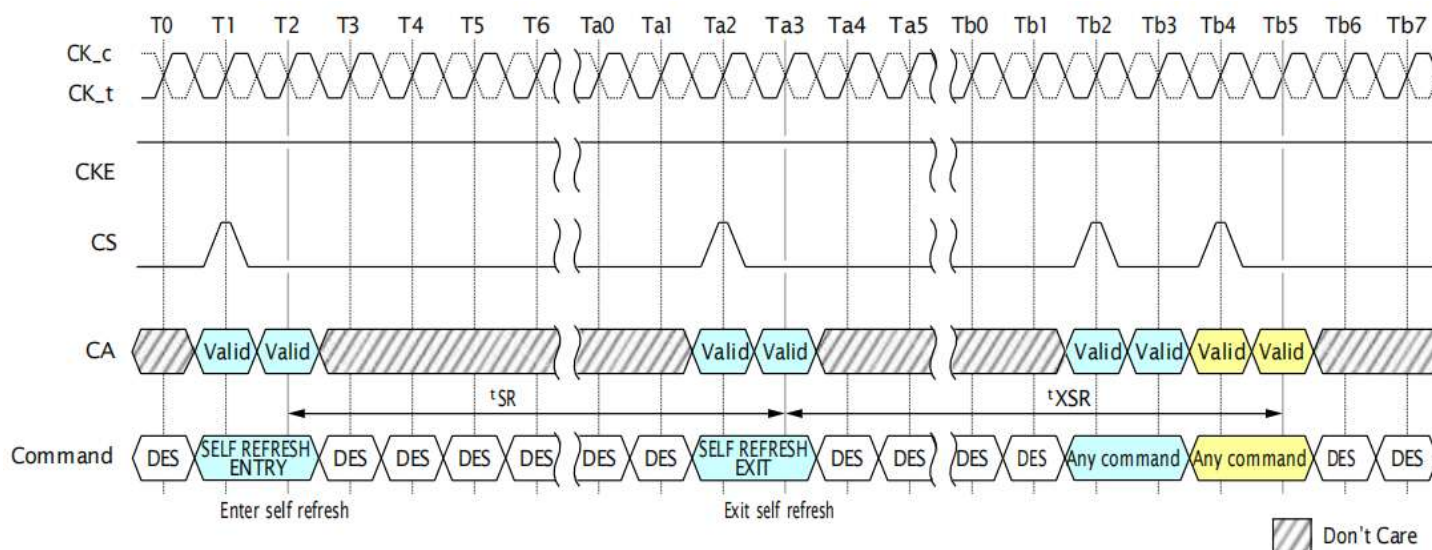
Figure 79: Self Refresh Entry/Exit Timing
