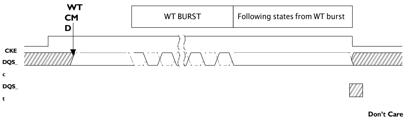
Figure 38: WDQS Control Mode 1
