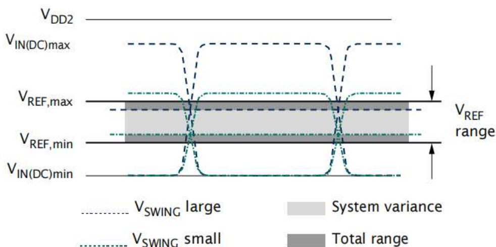
Figure 101: V_{REF} Operating Range ( V_{REF,max} , V_{REF,min} )
