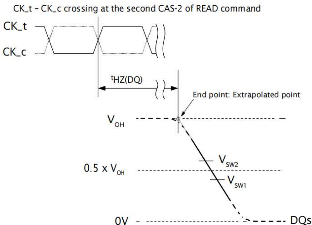
Figure 28: t_{HZ}(DQ) Method for Calculating Transitions and Endpoint
