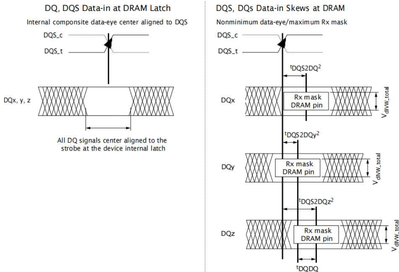
Figure 178: DQ-to-DQS t_{DQS2DQ} and t_{DQDQ}
