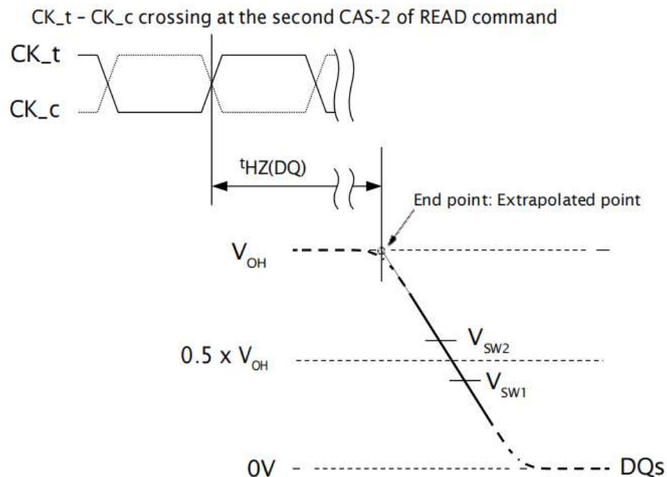
Figure 184: t_{HZ}(DQ) Method for Calculating Transitions and Endpoint
