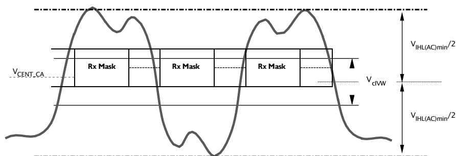
Figure 174: CA V_{IHL\_AC} Definition (for Each Input Pulse)
