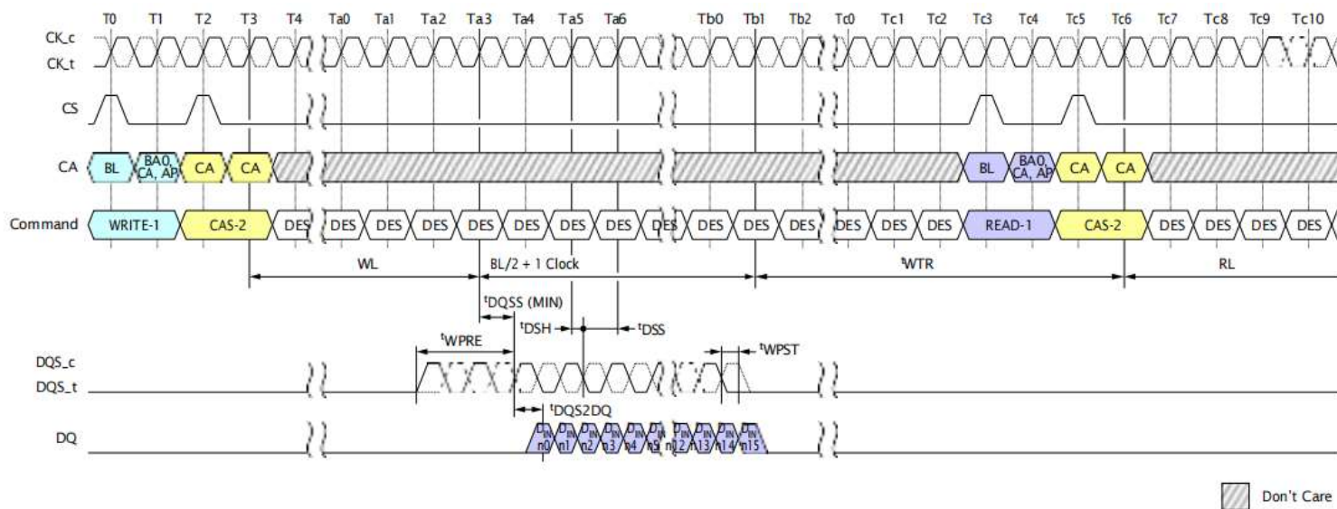
Figure 30: Burst Write Followed by Burst Read
