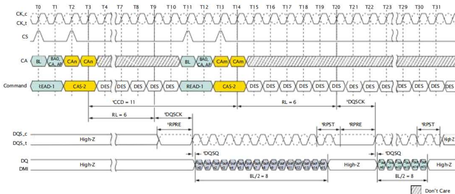
Figure 53: Consecutive READ: t_{CCD} = MIN + 3 , Preamble = Static, 1.5nCK Postamble
