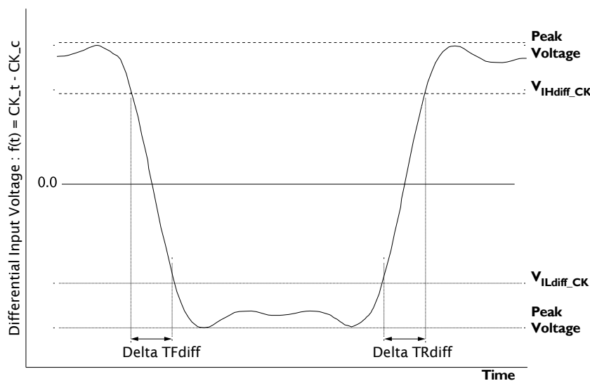
Figure I60: Differential Input Slew Rate Definition for DQS t , DQS c
