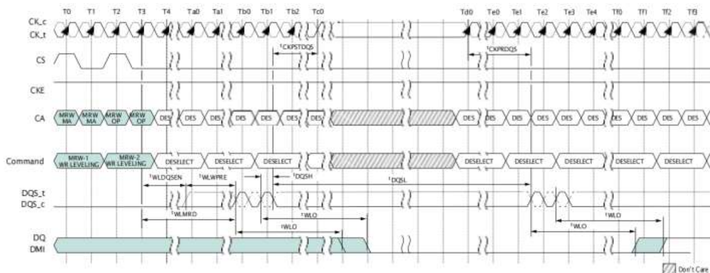
Figure 121: Clock Stop and Timing During Write Leveling
