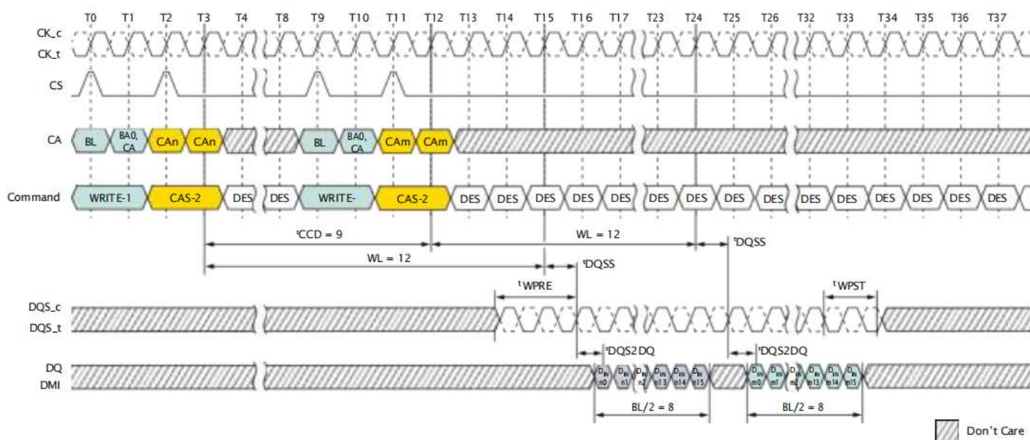
Figure 59: Consecutive WRITE: t_{CCD} = \text{MIN} + 1, 1.5n\text{CK} Postamble
