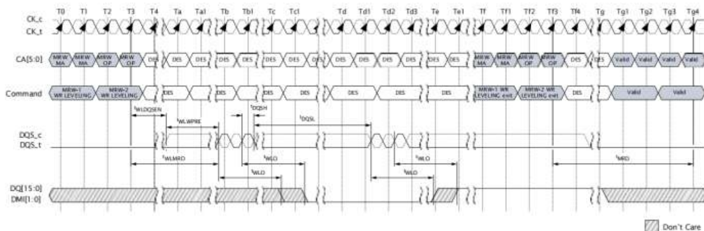
Figure I 19: Write Leveling Timing – ‘DQSL(MAX)
