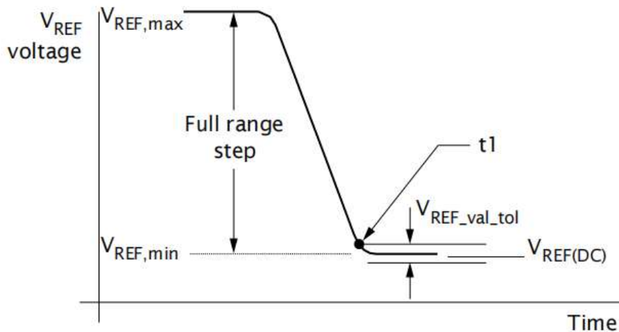
Figure I07: V_{REF(CA)} Full Step from V_{REF,max} to V_{REF,min}
