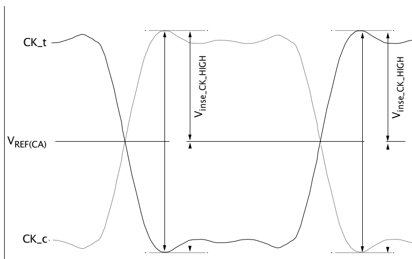
Figure I54: Clock Single-Ended Input Voltage
