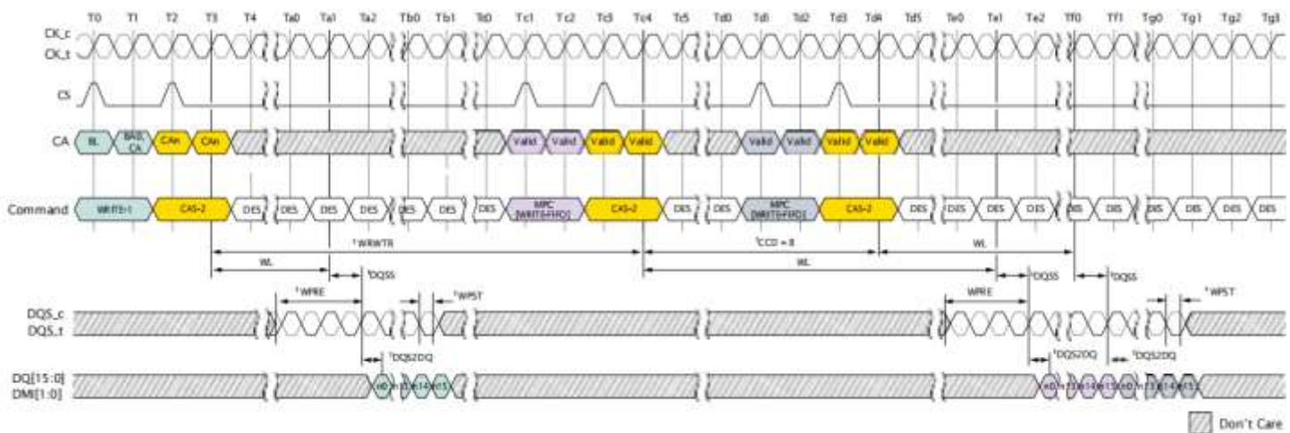
Figure 129: WRITE-to-MPC[WRITE-FIFO] Operation Timing
