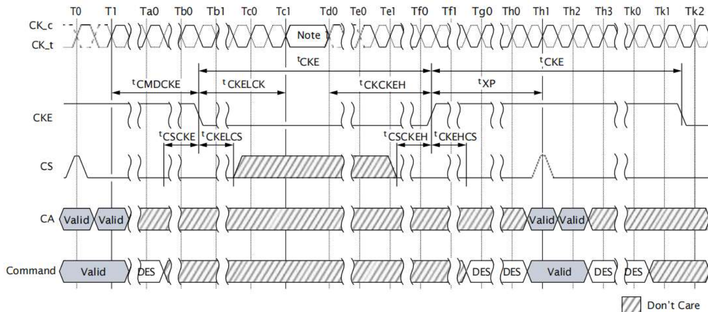
Figure 84: Basic Power-Down Entry and Exit Timing
