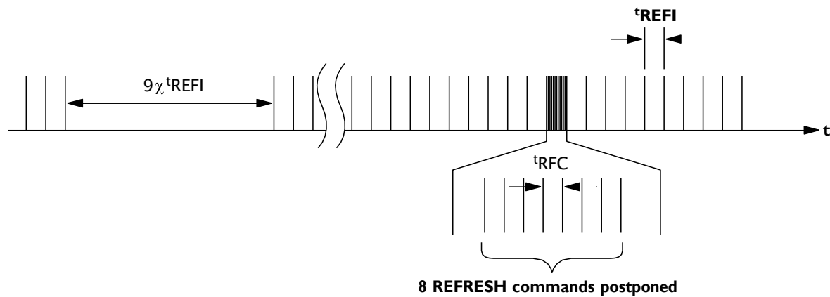
Figure 75: Postponing REFRESH Commands (Example)
