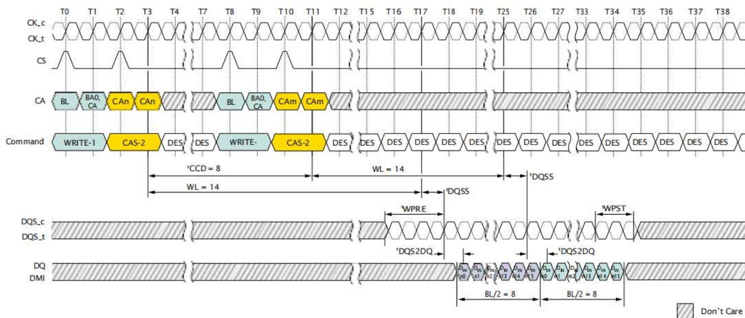
Figure 57: Seamless WRITE: t_{CCD} = \text{MIN} , 1.5nCK Postamble
