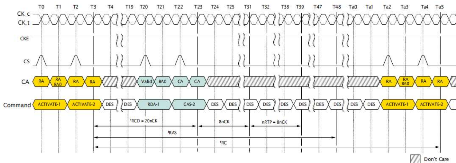
Figure 71: Command Input Timing with RAS Lock
