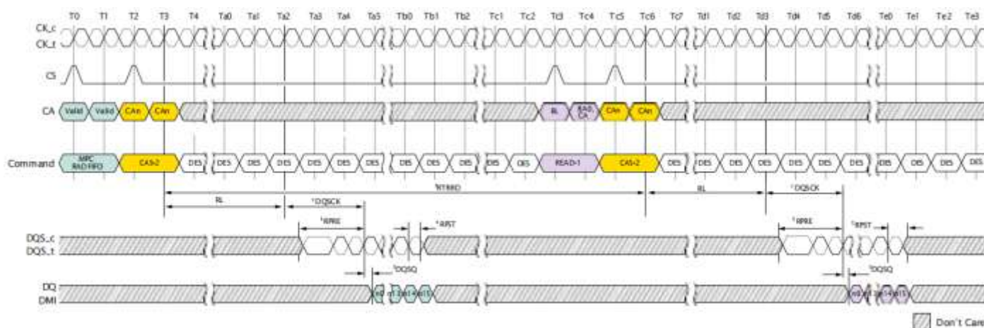
Figure 131: MPC[READ-FIFO] to Read Timing
