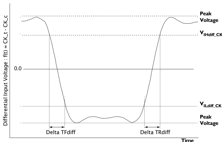
Figure I 55: Differential Input Slew Rate Definition for CK t , CK c
