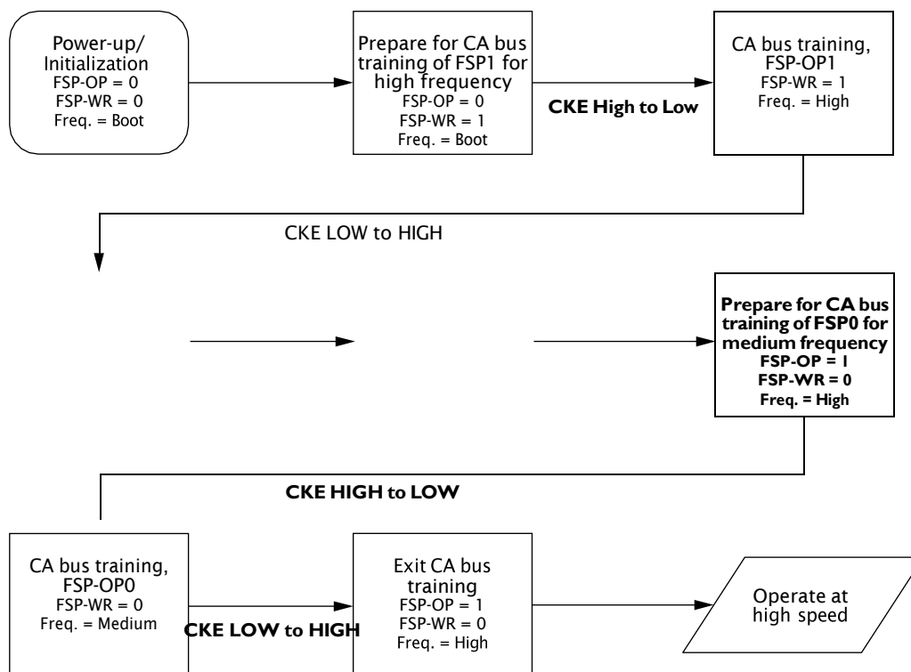
Figure I40: Training for Two Frequency Set Points
