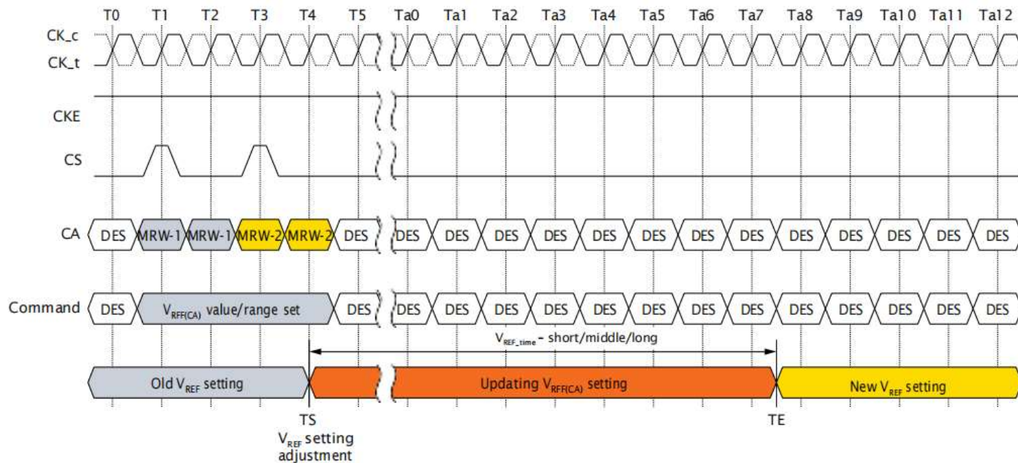
Figure I03: t_{V_{ref}} for Short, Middle, and Long Timing Diagram
