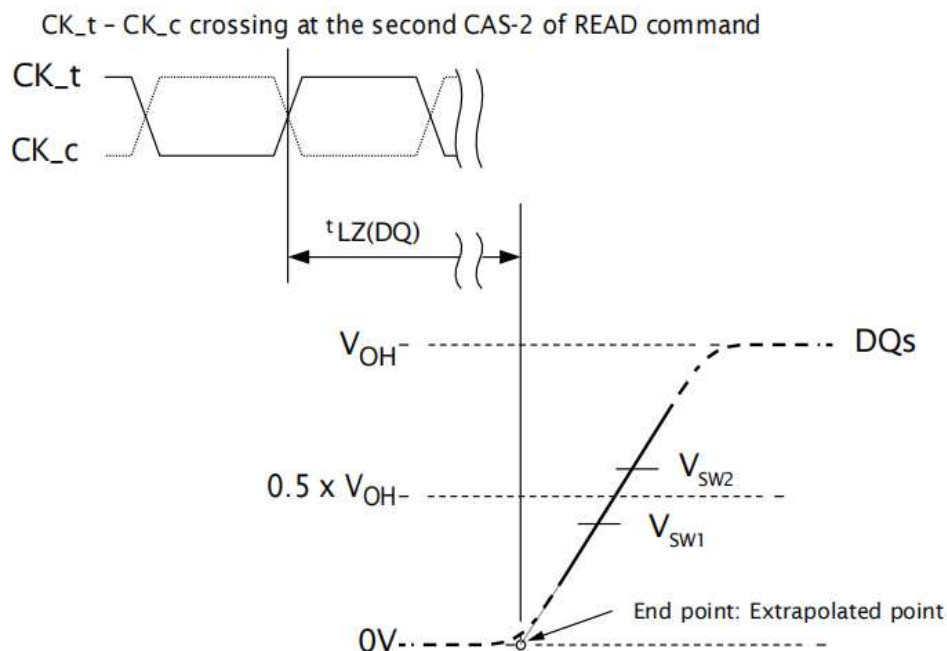
Figure 27: t_{LZ}(DQ) Method for Calculating Transitions and Endpoint
