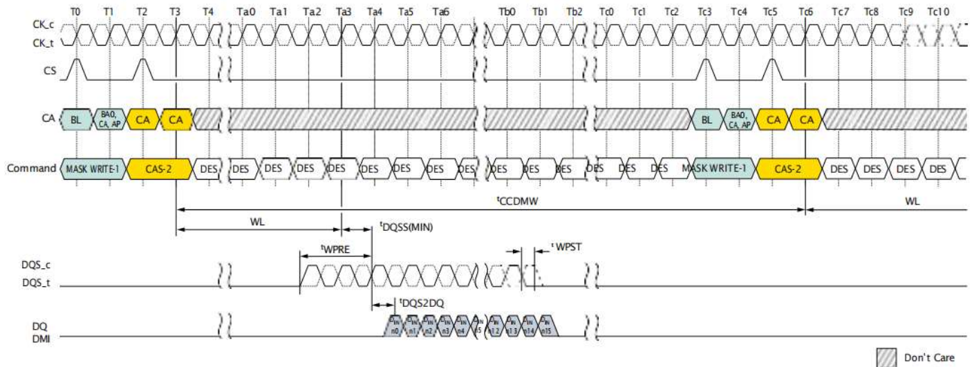
Figure 34: MASK WRITE Command – Same Bank
