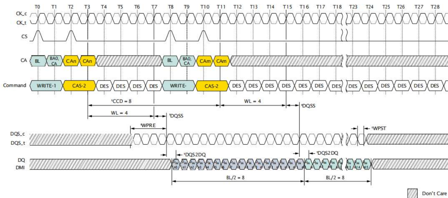
Figure 55: Seamless WRITE: t_{CCD} = \text{MIN}, 0.5n\text{CK} Postamble
