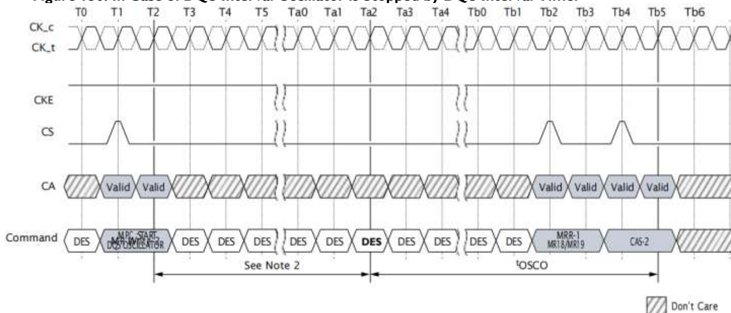
Figure I36: In Case of DQS Interval Oscillator is Stopped by DQS Interval Timer
