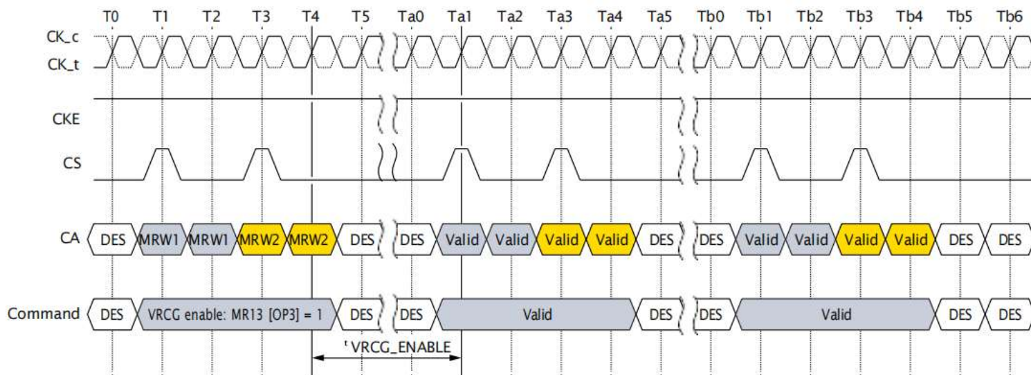
Figure 99: VRCG Enable Timing
