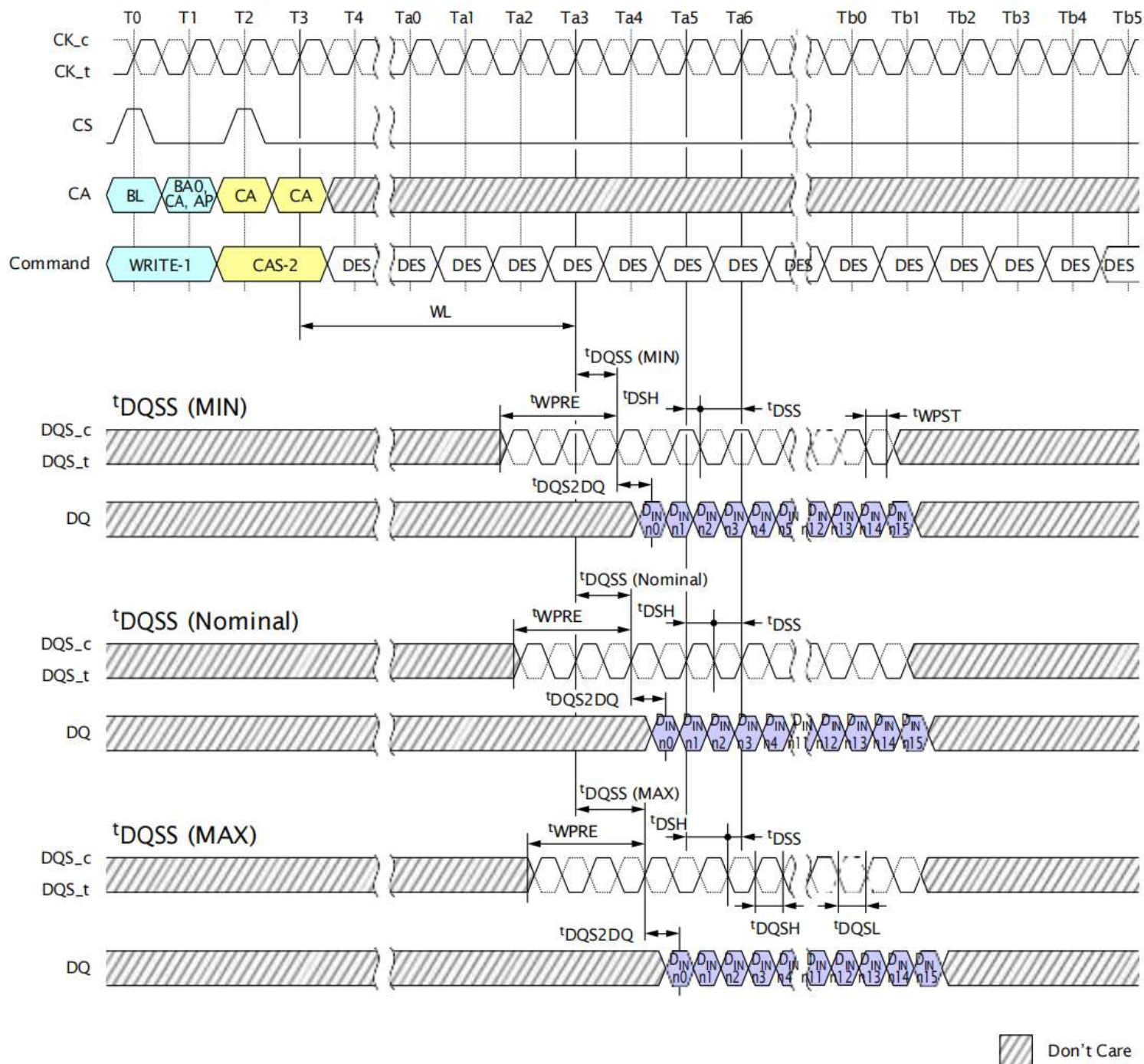
Figure 31: Write Timing
