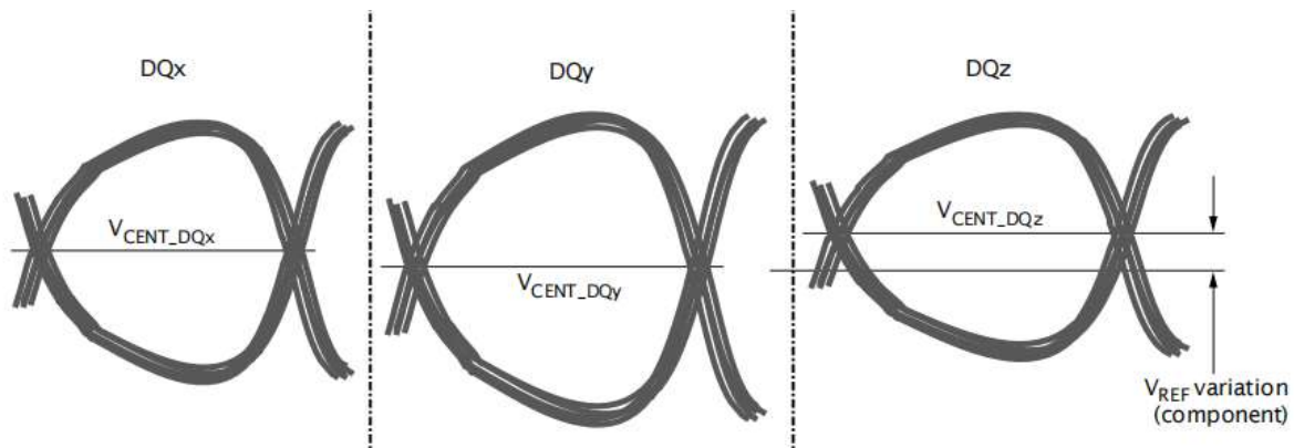
Figure 177: Across Pin V_{REF} DQ Voltage Variation
