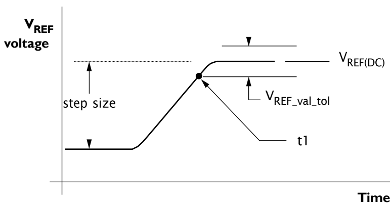
Figure I04: V_{REF(CA)} Single-Step Increment
