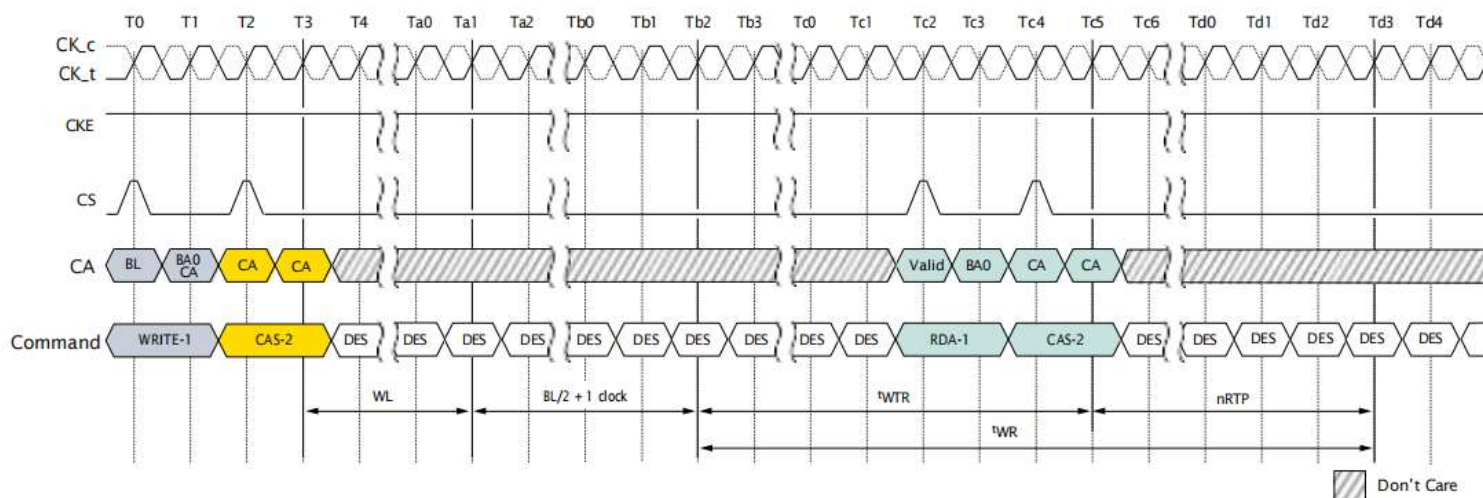
Figure 72: Delay Time From WRITE-to-READ with Auto Precharge
