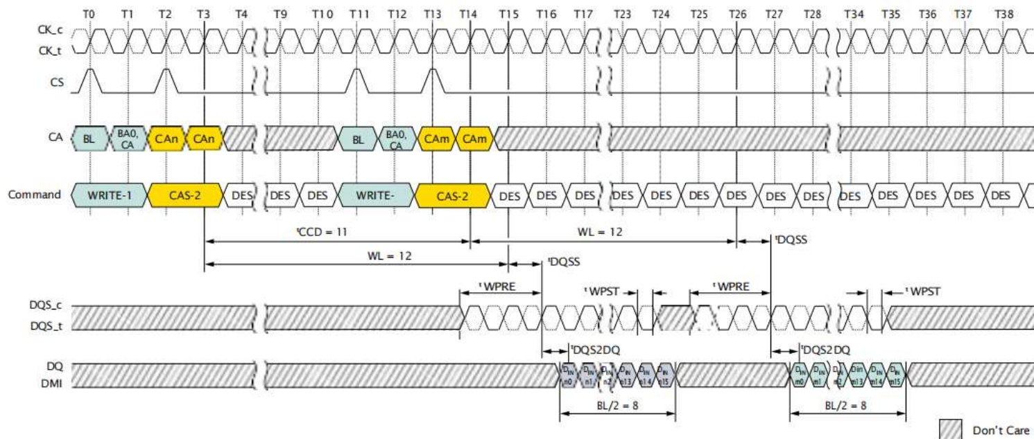
Figure 62: Consecutive WRITE: t_{CCD} = MIN + 3, 0.5nCK Postamble
