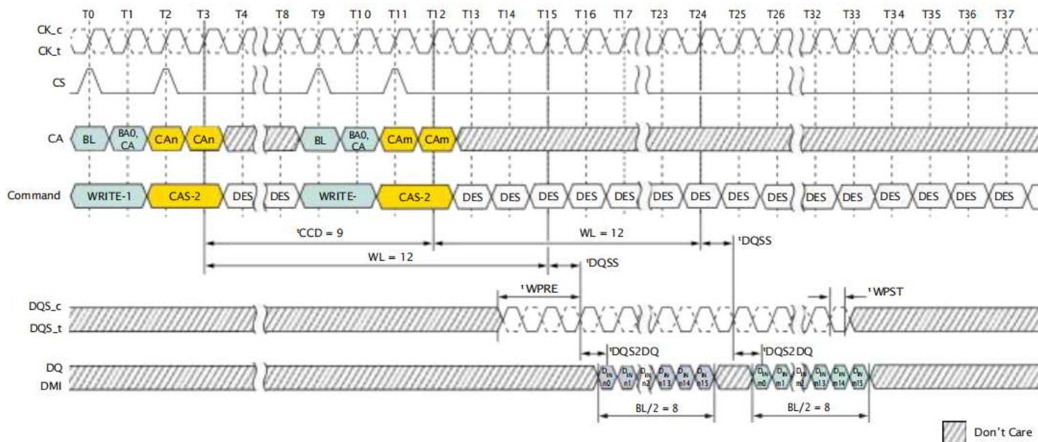
Figure 58: Consecutive WRITE: t_{CCD} = \text{MIN} + 1, 0.5n\text{CK} Postamble
