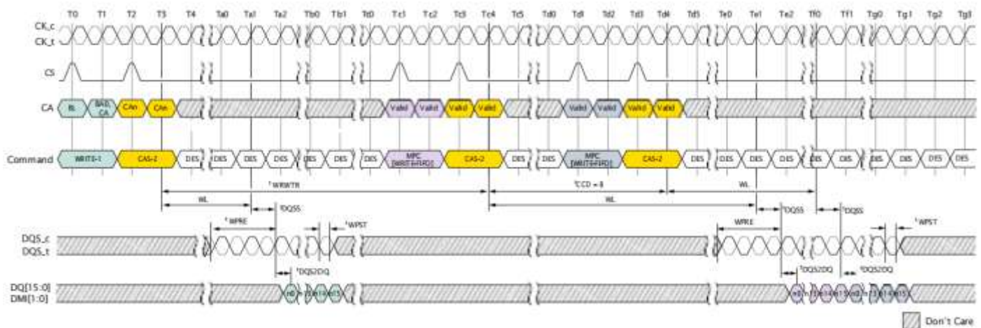
Figure 123: WRITE-FIFO – t_{WPRE} = 2nCK , t_{WPST} = 0.5nCK
