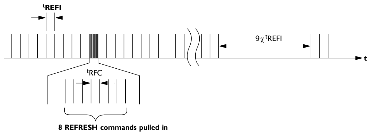
Figure 76: Pulling in REFRESH Commands (Example)
