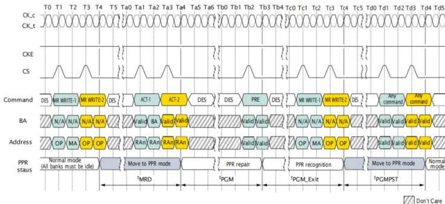
Figure I48: Post-Package Repair Timing
