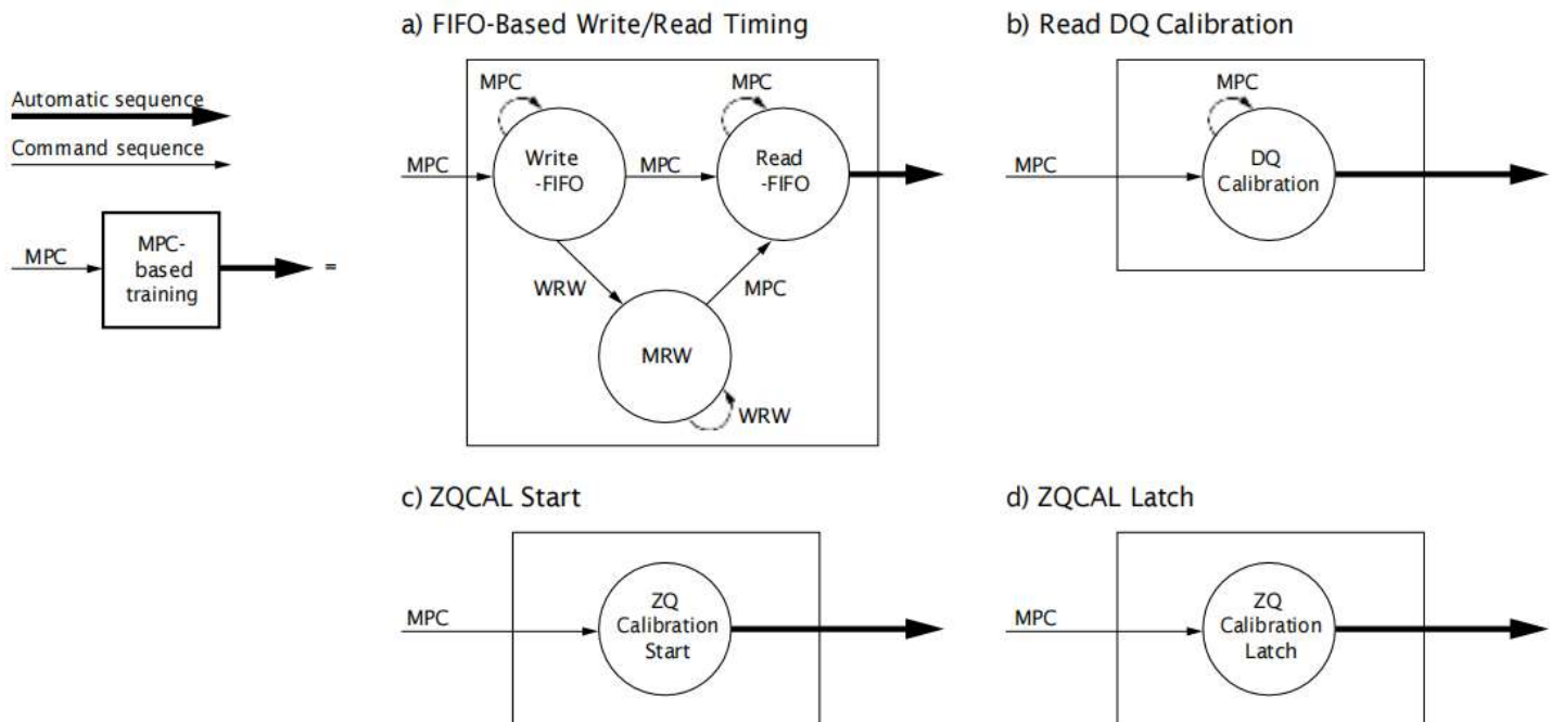
Figure 13: Simplified State Diagram
