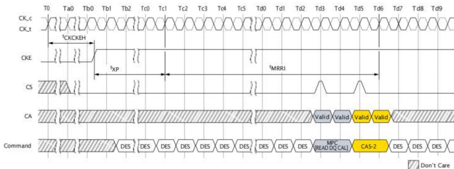
Figure 128: MPC[READ DQ CALIBRATION] Following Power-Down State
