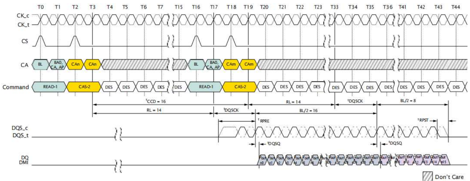
Figure 21: Burst Read Timing
