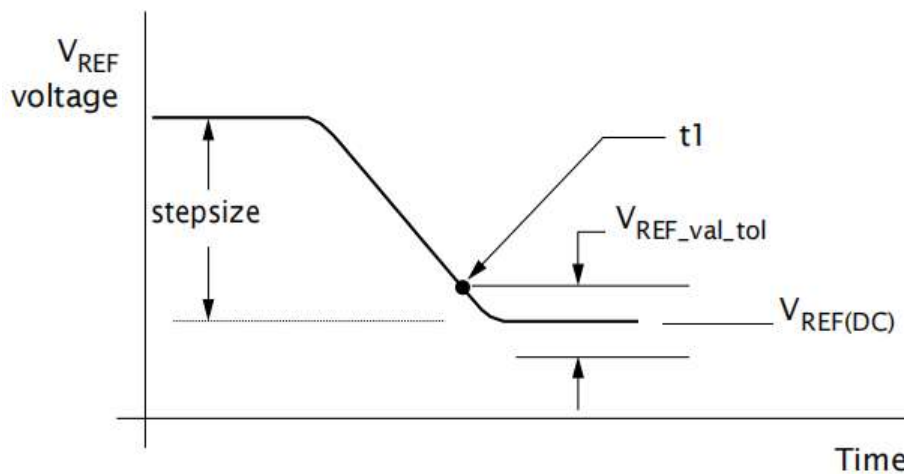
Figure 113: V_{REF(DQ)} Full Step from V_{REF,min} to V_{REF,max}
