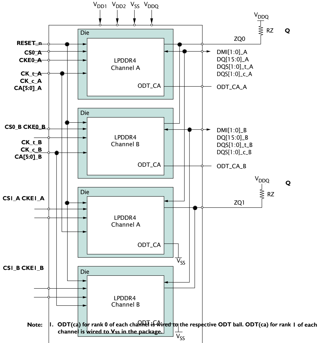
Figure 4: Quad-Die, Dual-Channel, Dual-Rank Package Block Diagram (x32 I/O)
