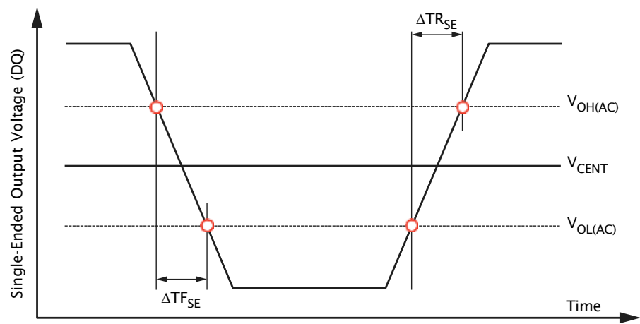
Figure I87: Single-Ended Output Slew Rate Definition
