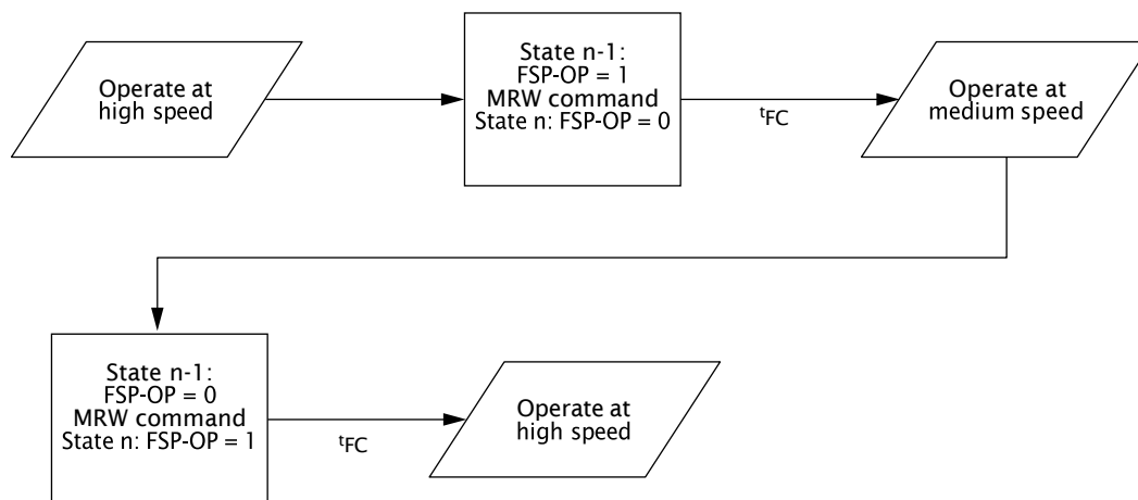
Figure I41: Example of Switching Between Two Trained Frequency Set Points
