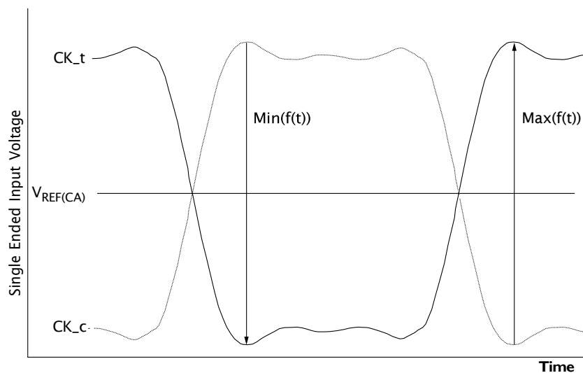
Figure I53: Definition of Differential Clock Peak Voltage
