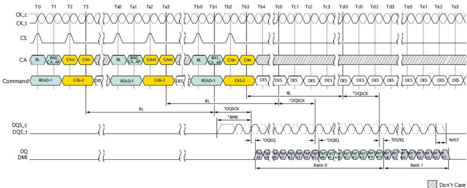
Figure 23: Seamless Burst Read
