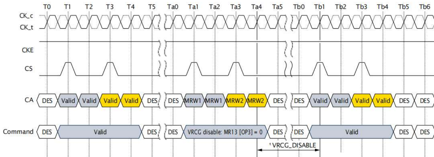
Figure 100: VRCG Disable Timing
