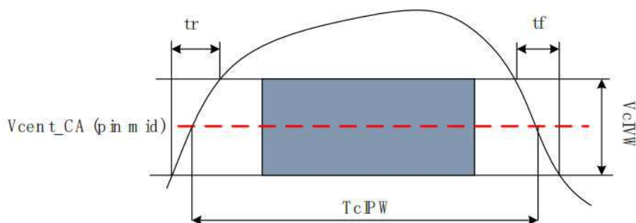
Figure 8-4 CA TcIPW and SRIN_cIWV definition (for each input pulse)
