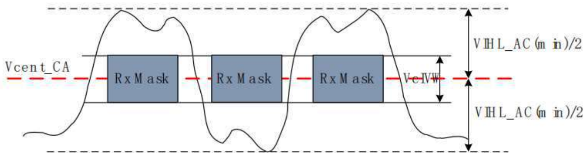
Figure 8-5 CA VIH_L_AC Definition (for Each Input Pulse)
