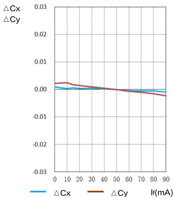
色坐标数据表/Chromaticity coordinate shift \Delta C_x, \Delta C_y = f(I_f); T_s = 25^\circ\text{C}
