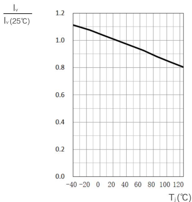
相对发光强度 / Relative Luminous Intensity I_v/I_v(25^\circ\text{C}) = f(T_j); I_f = 50\text{ mA}
